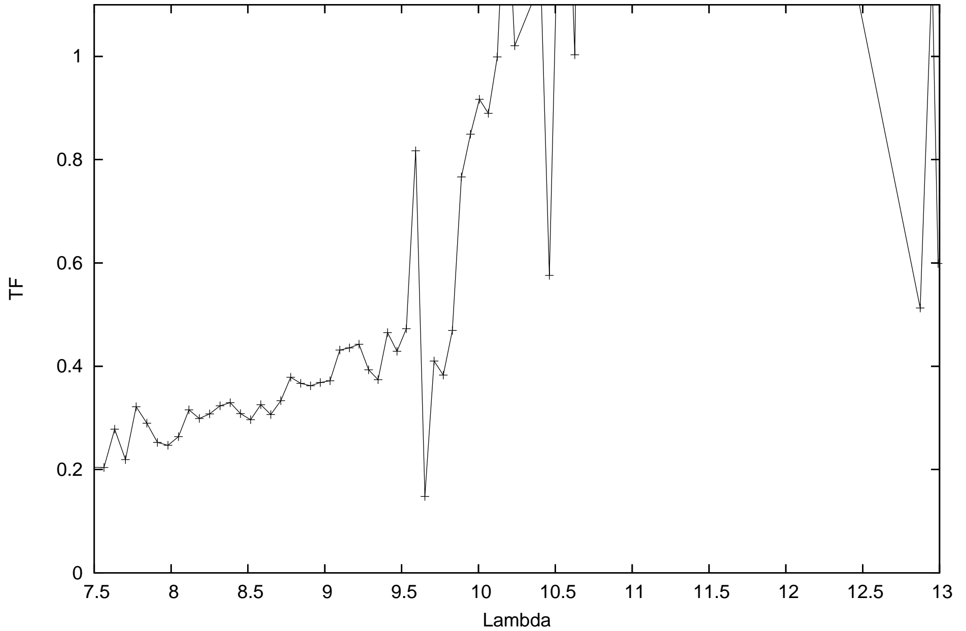
calHD224935_flux-0.85_diam7.24_r.MIDI.2011-08-11T09_18_47.015_B2A1
