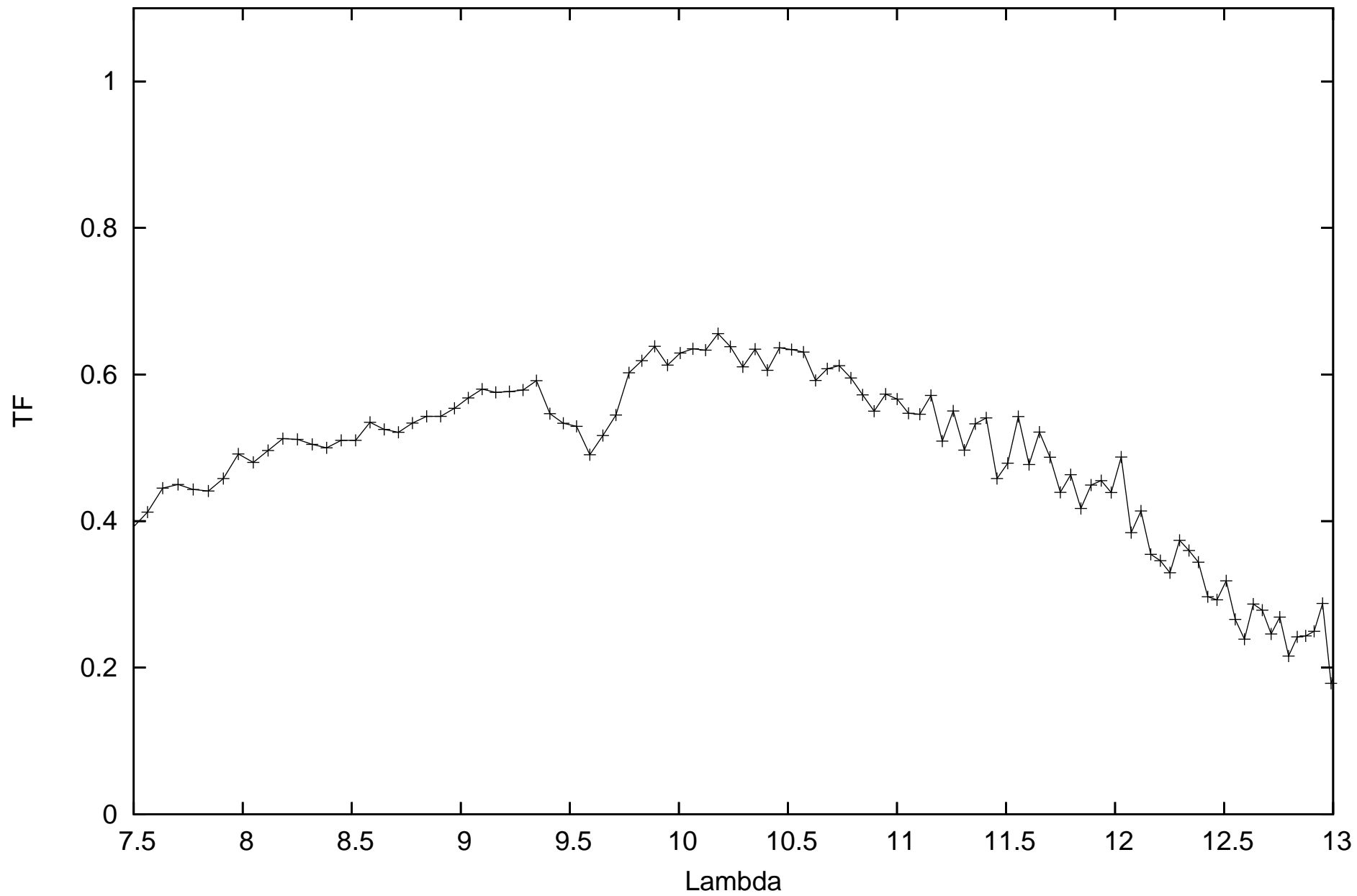
calHD206778_flux-1.04_diam7.59_r.MIDI.2011-08-11T07_19_59.015_C1A1
