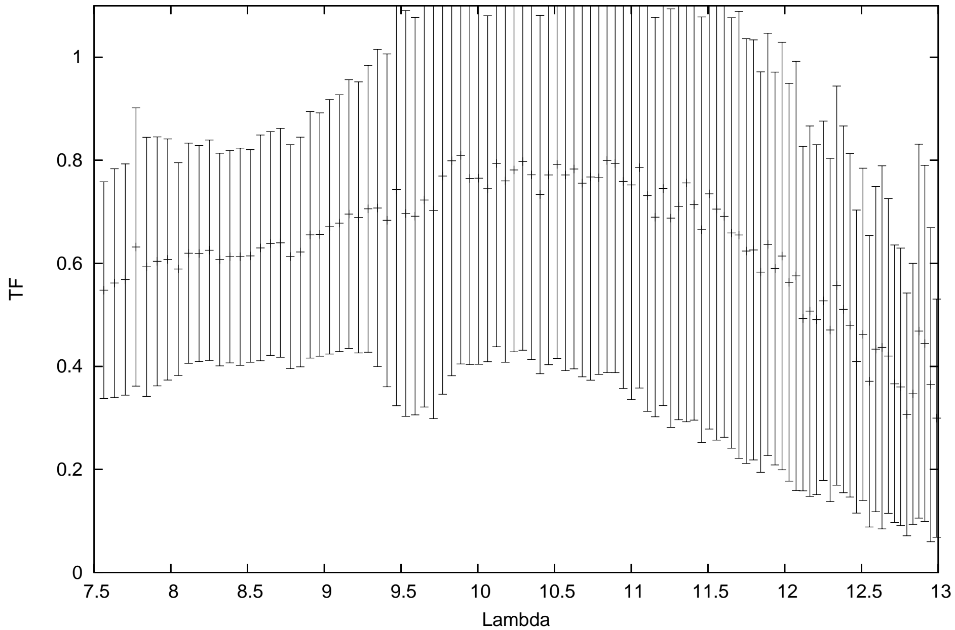
calHD206778_flux-1.04_diam7.59_r.MIDI.2011-08-11T06_41_14.015_C1A1
