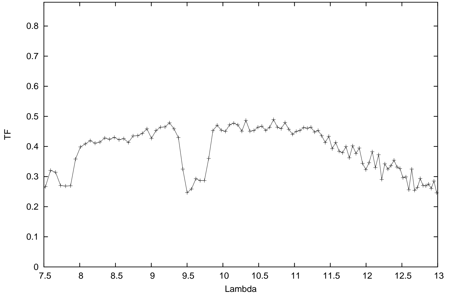
calHIP90496_flux0.238088_diam3.99_r.MIDI.2011-06-29T09_23_28.000_H011
