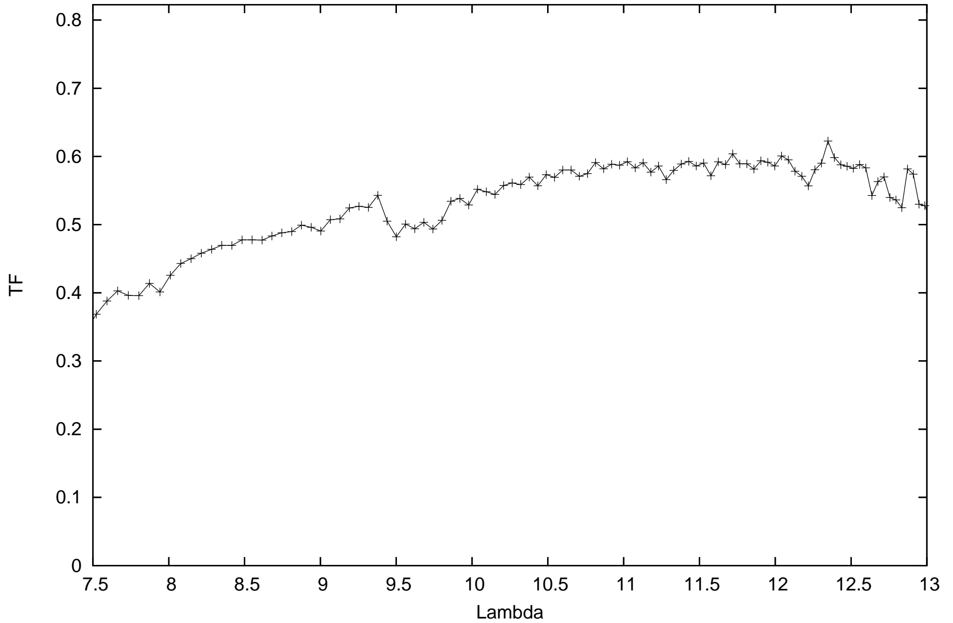
calHIP89931_flux-0.511_diam5.87_r.MIDI.2011-06-29T08_35_10.000_H011
