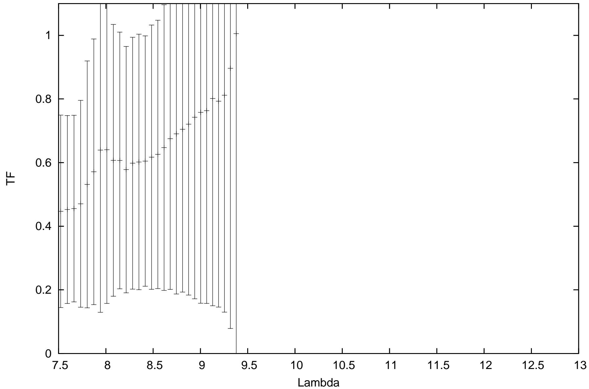
calHIP89931_flux-0.511_diam5.87_r.MIDI.2011-06-26T08_26_08.000_G111
