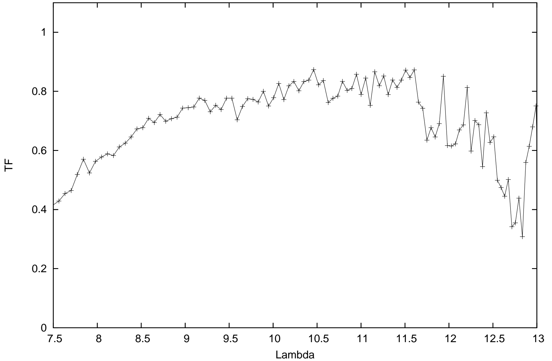
calHD206778_flux-1.04_diam7.59_r.MIDI.2011-06-12T08_50_03.945_B2A1
