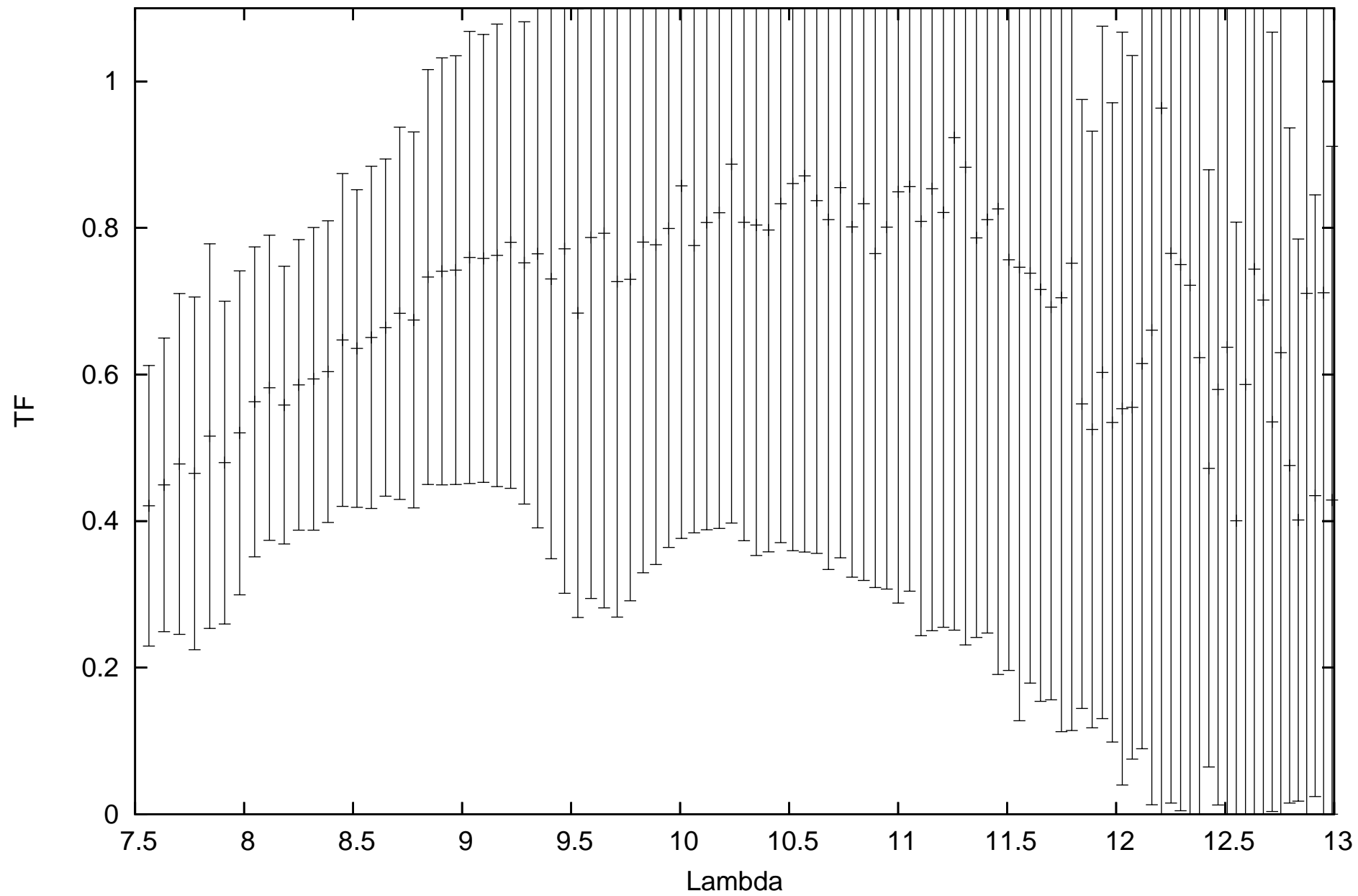
calHD206778_flux-1.04_diam7.59_r.MIDI.2011-06-12T08_20_08.110_B2A1
