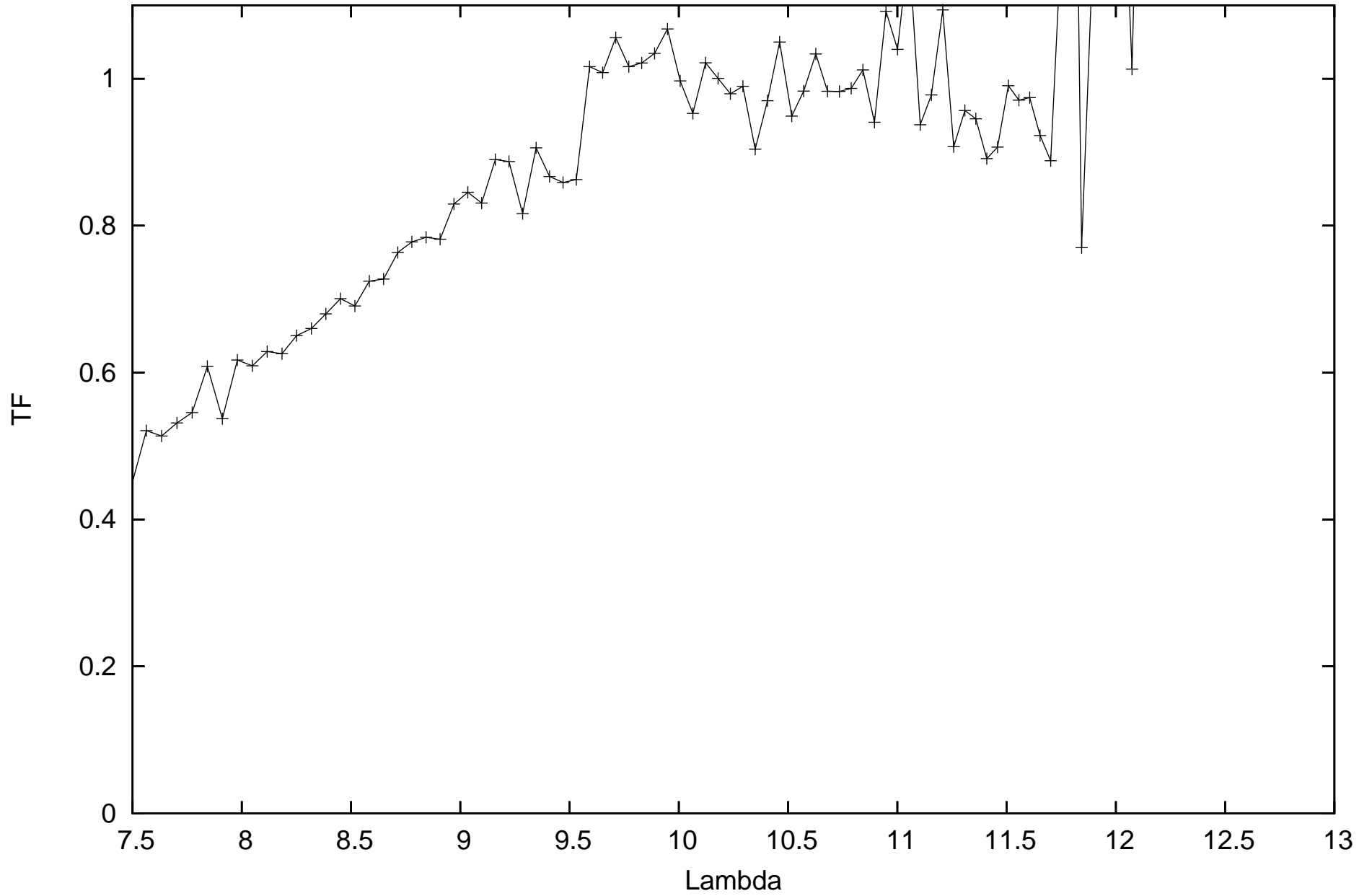
calHD206778_flux-1.04_diam7.59_r.MIDI.2011-06-12T08_06_55.946_B2A1
