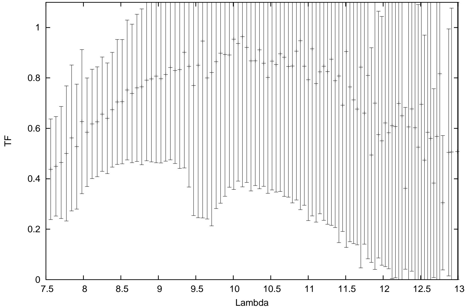
calHD206778_flux-1.04_diam7.59_r.MIDI.2011-06-12T07_36_39.946_B2A1
