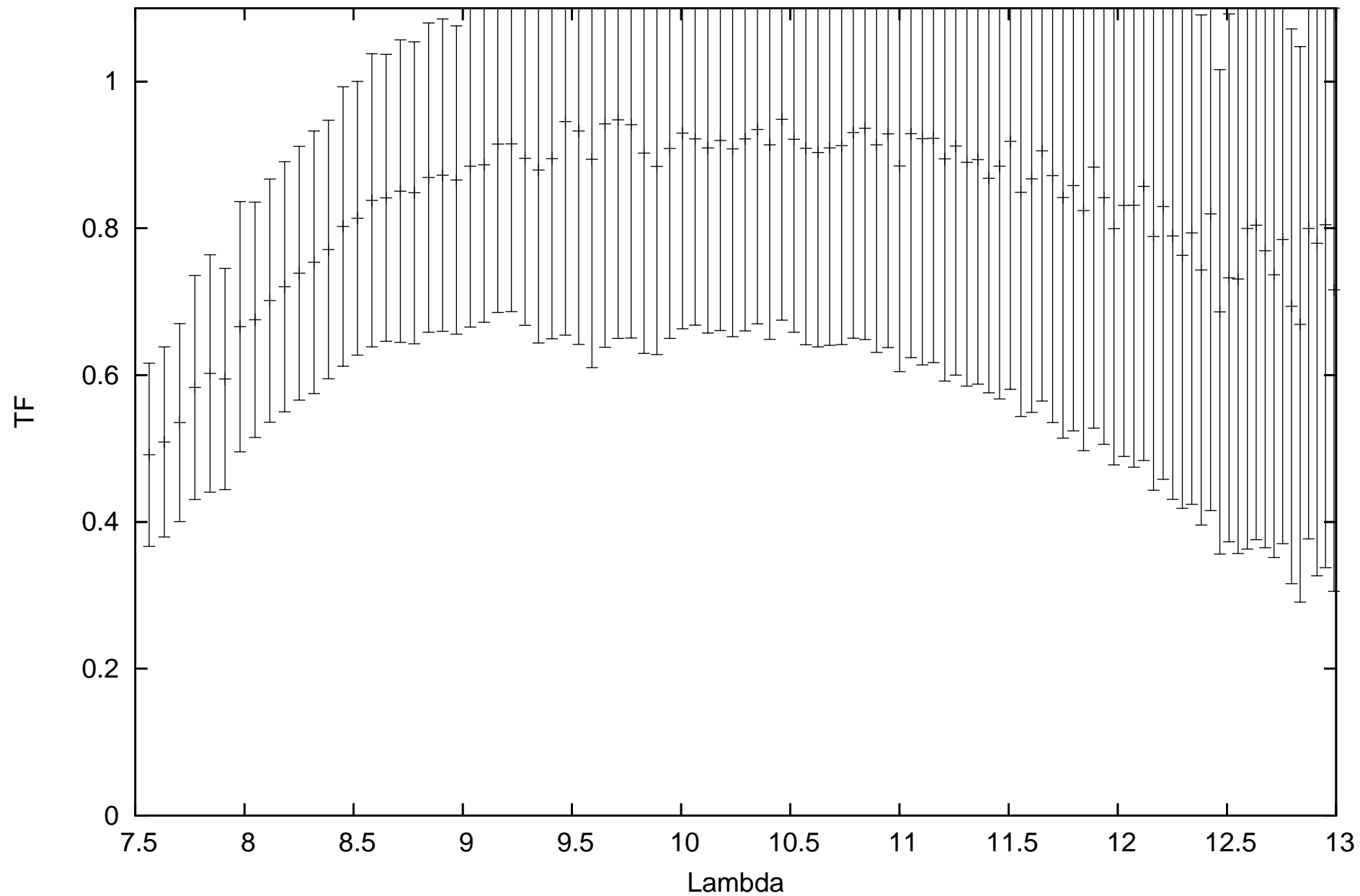
calHD167618_flux-1.82_diam11.66_r.MIDI.2011-06-12T07_02_43.015_B2A1
