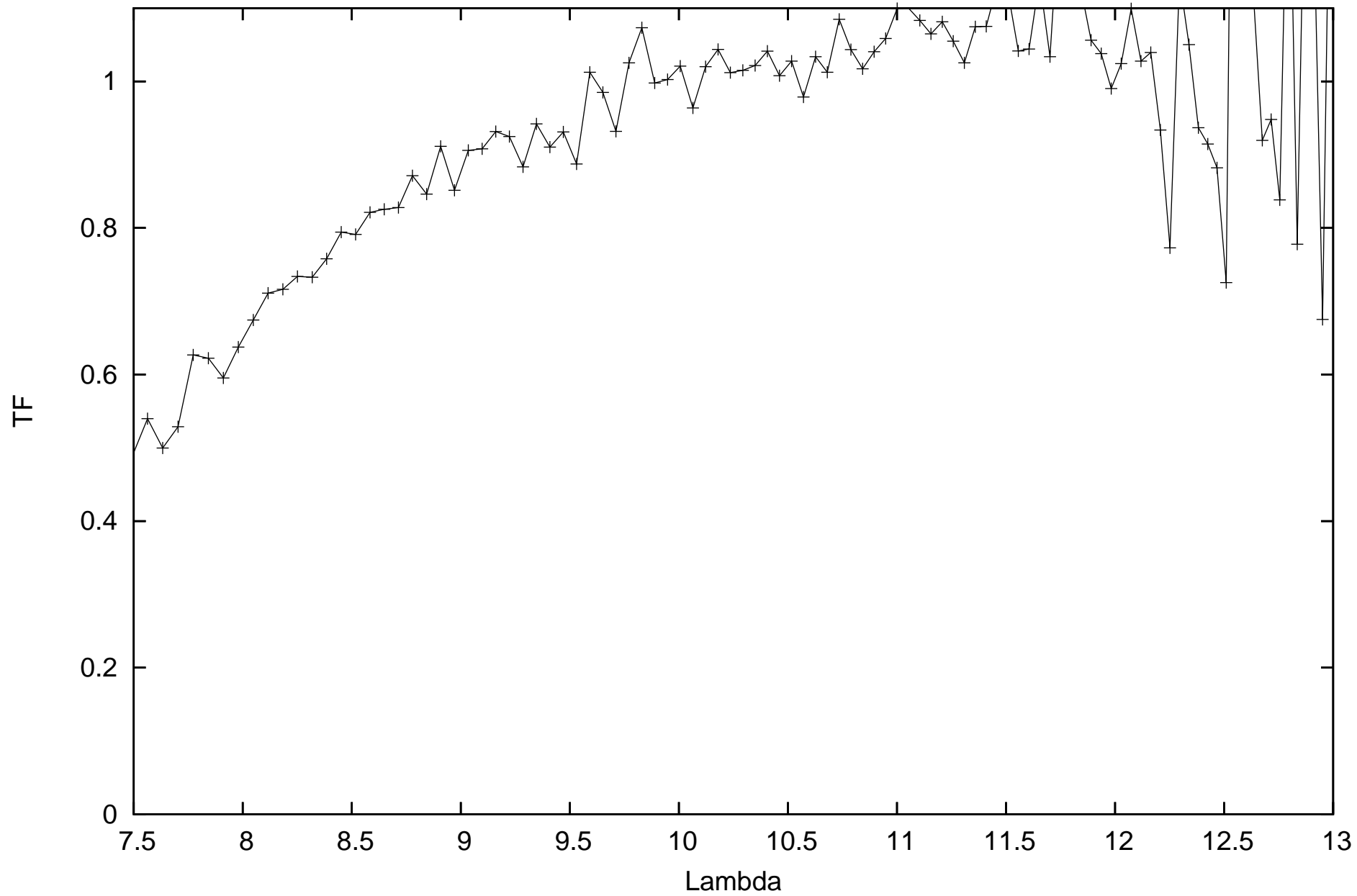
calHIP83081_flux-0.81238_diam6.88_r.MIDI.2011-06-11T01_38_38.015_C1A1
