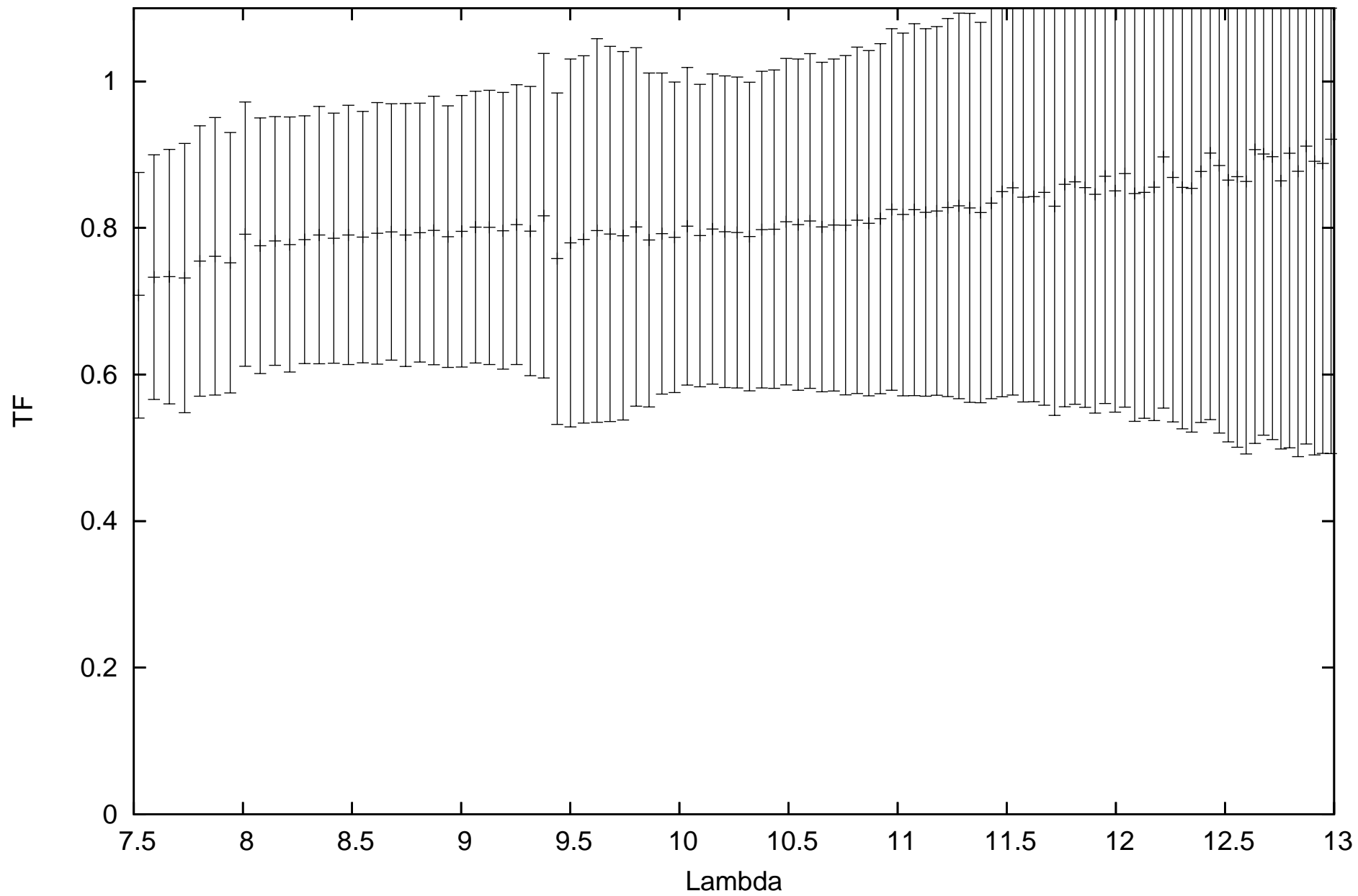
calHD167618_flux-1.82_diam11.66_r.MIDI.2011-06-11T10_10_44.000_C1B2
