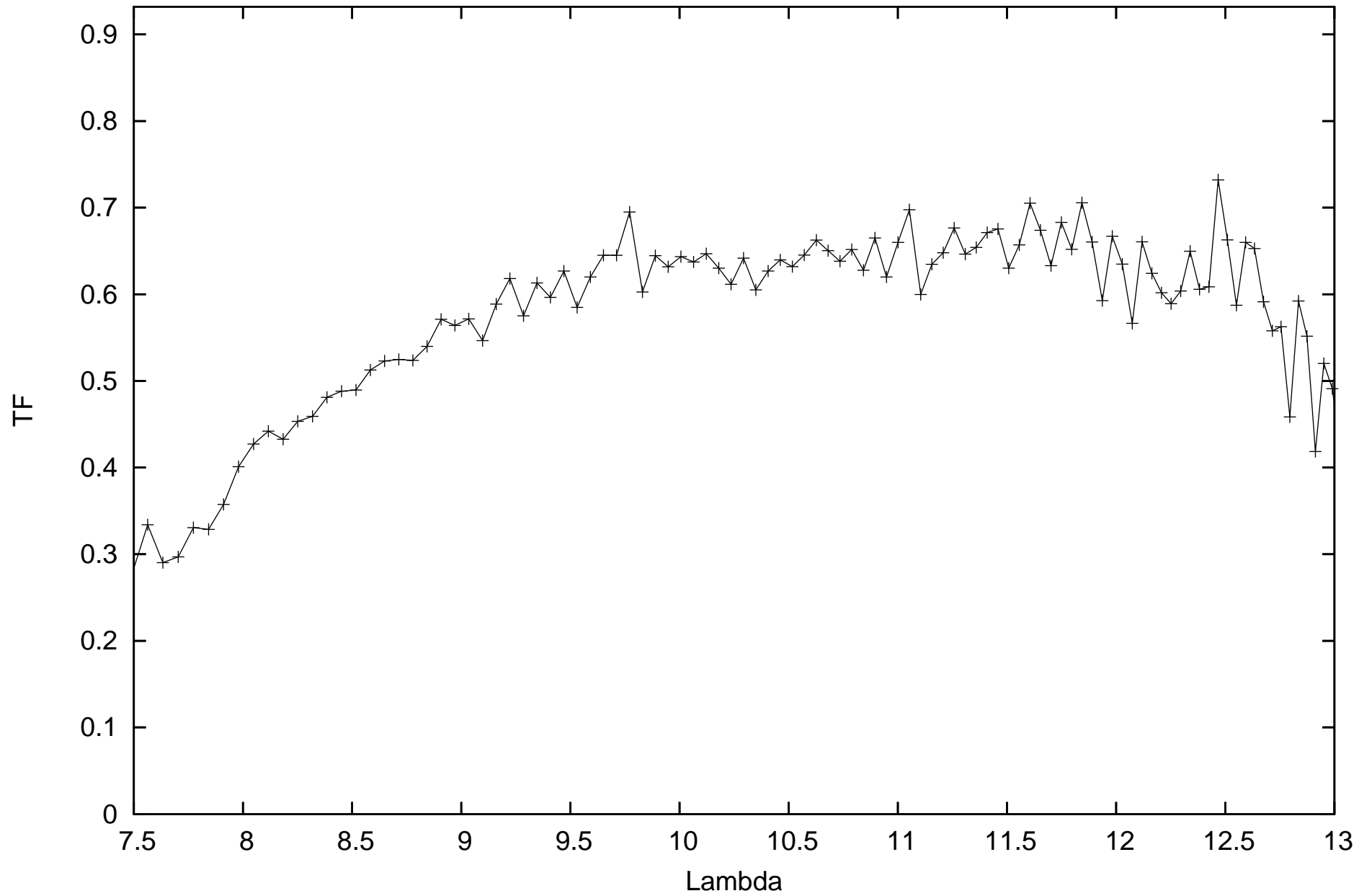
calHD167618_flux-1.82_diam11.66_r.MIDI.2011-06-06T03_54_56.138_C1B2
