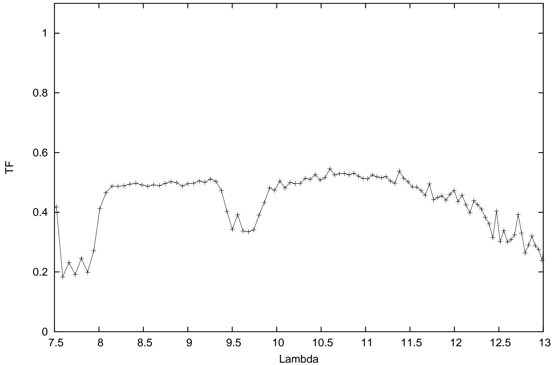
calHIP82363_flux-0.3207_diam5.52_r.MIDI.2011-05-30T10_15_22.000_DOG1
