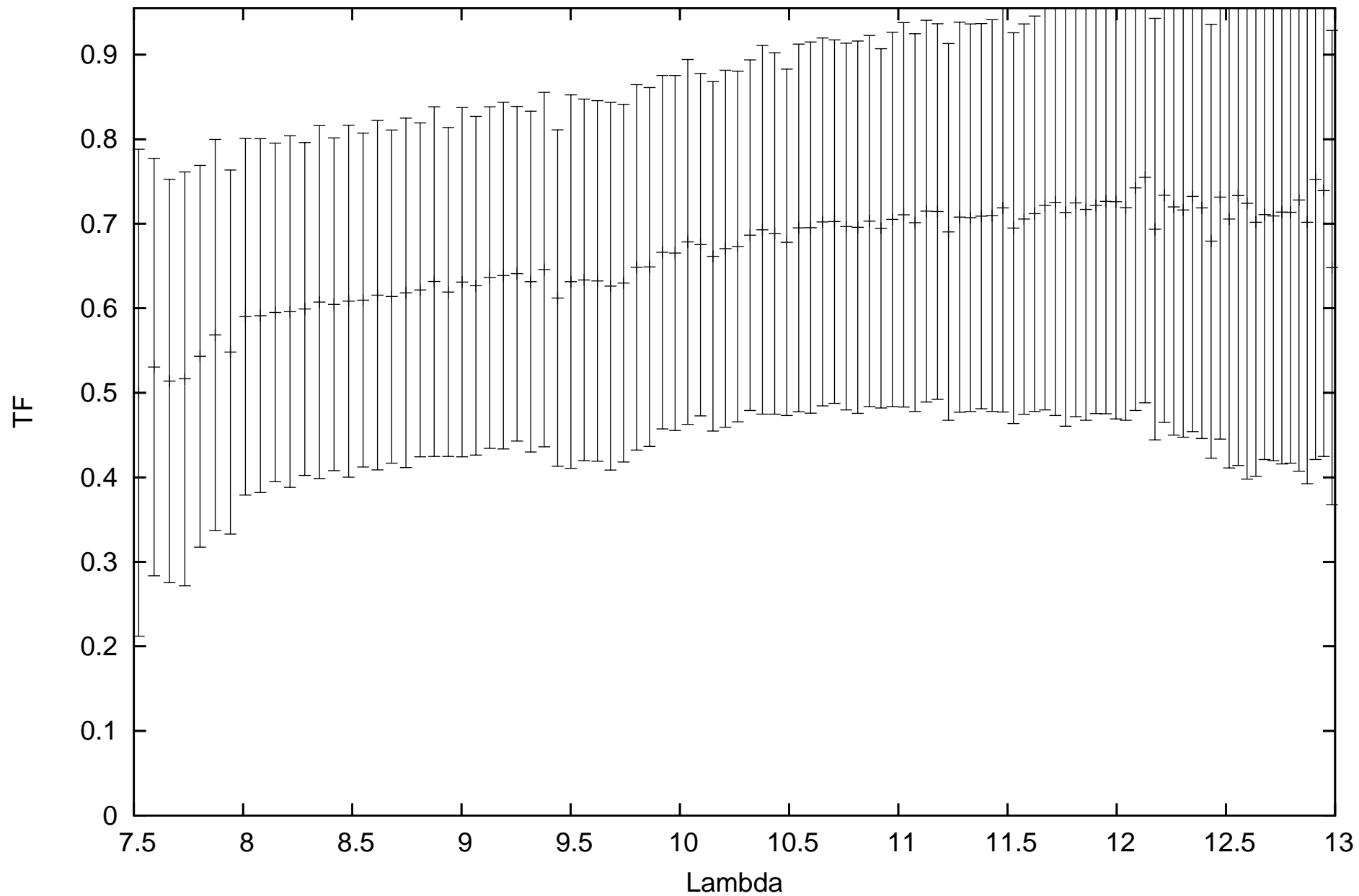
calHIP82273_flux-1.42243_diam8.91_r.MIDI.2011-05-30T06_55_42.000_D0H0
