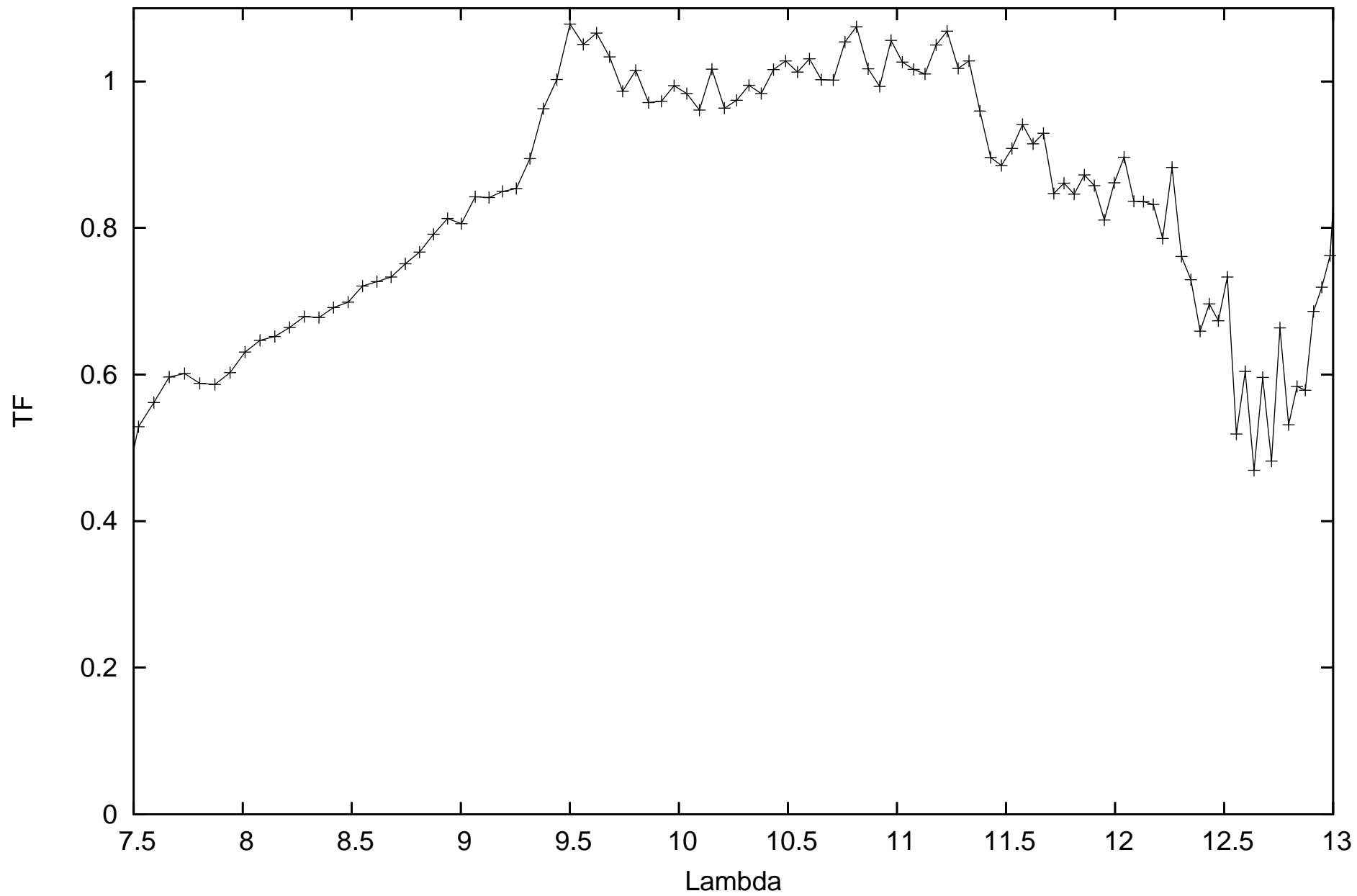
calHIP90496_flux0.238088_diam3.99_r.MIDI.2011-05-28T05_51_27.000_K011
