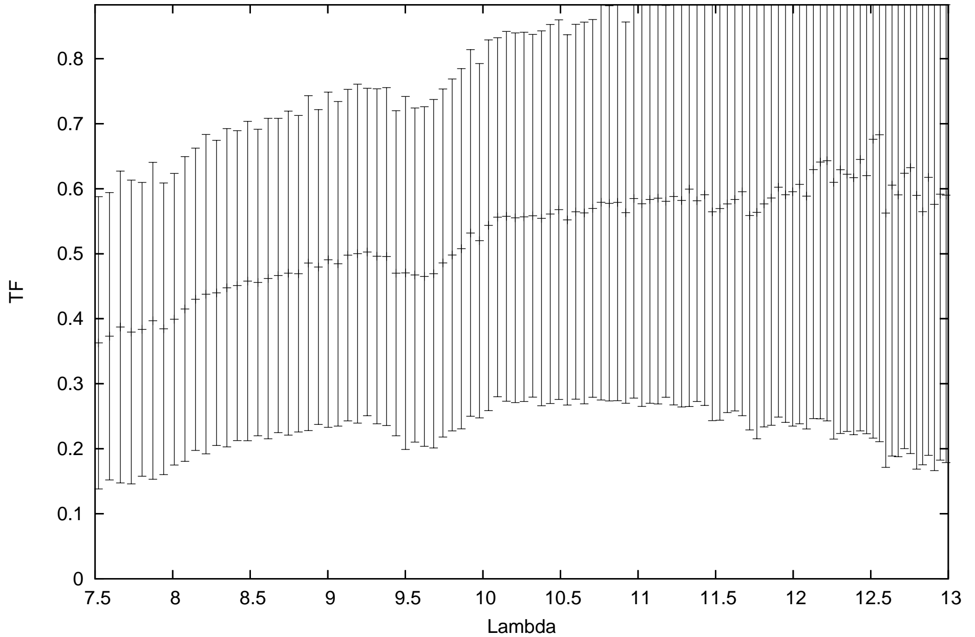
calHIP89931_flux-0.511_diam5.87_r.MIDI.2011-05-28T06_15_23.000_K011
