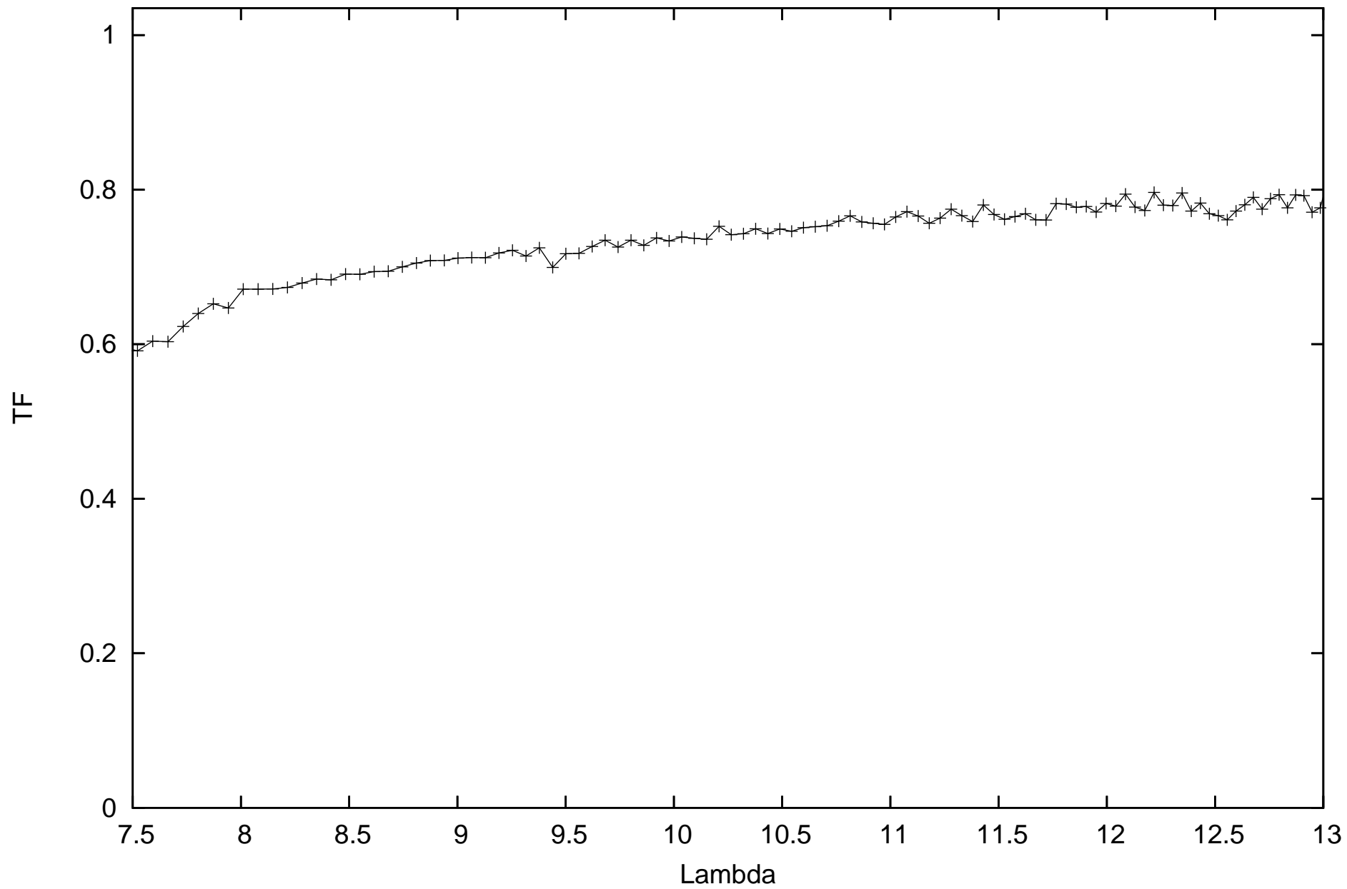
calHD157236_flux1.45_diam2.51_r.MIDI.2011-05-16T08_25_02.000_U2U3
