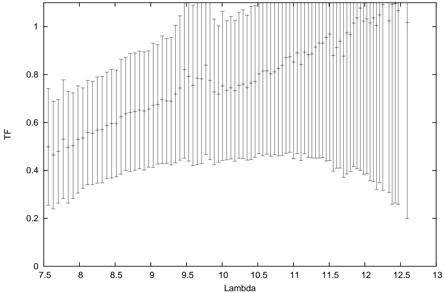
calHD167618_flux-1.82_diam11.66_r.MIDI.2011-05-10T06_58_10.138_B2A1
