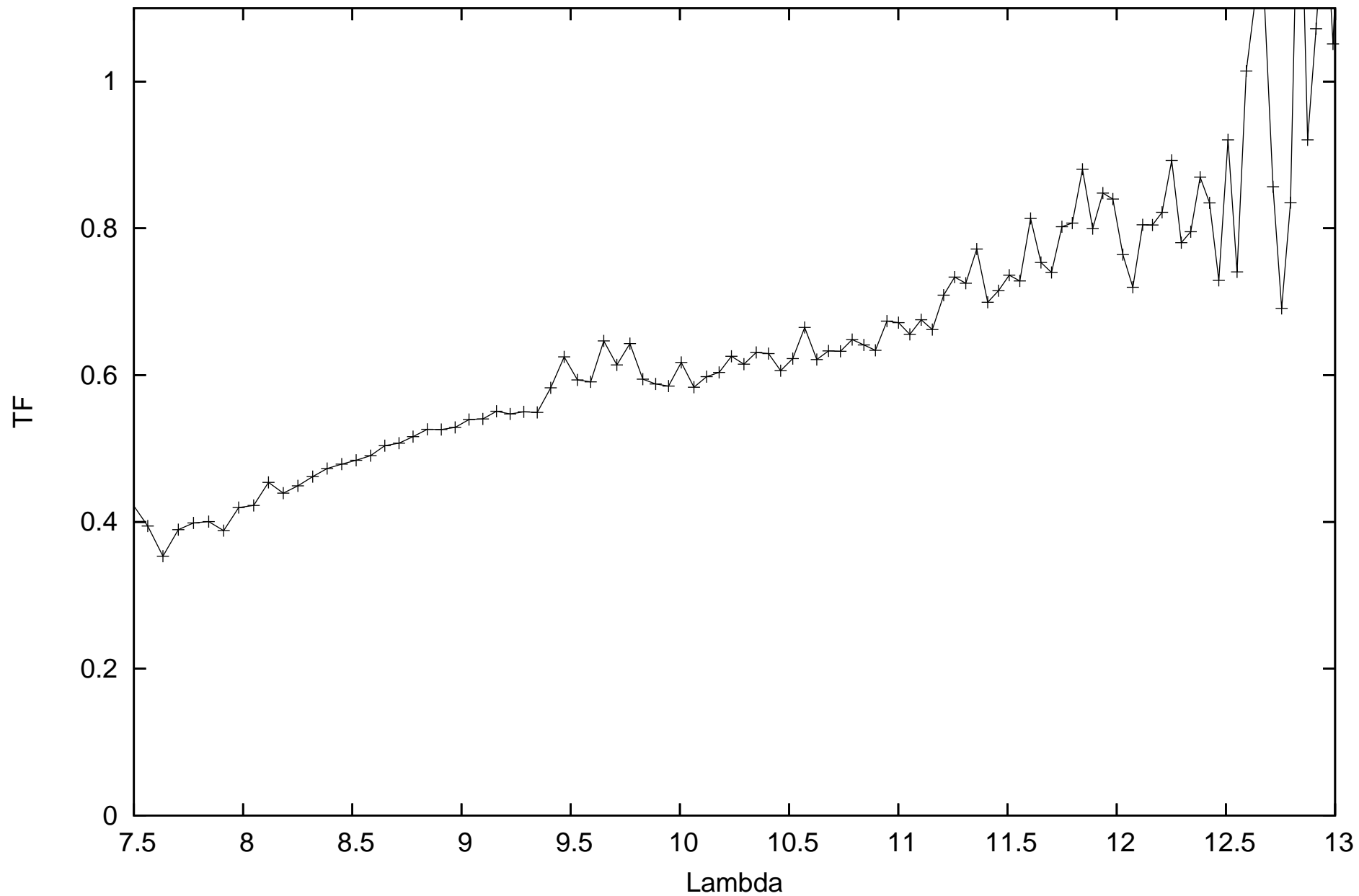
calHD120323_flux-2.02_diam13.25_r.MIDI.2011-05-10T04_25_46.179_B2A1
