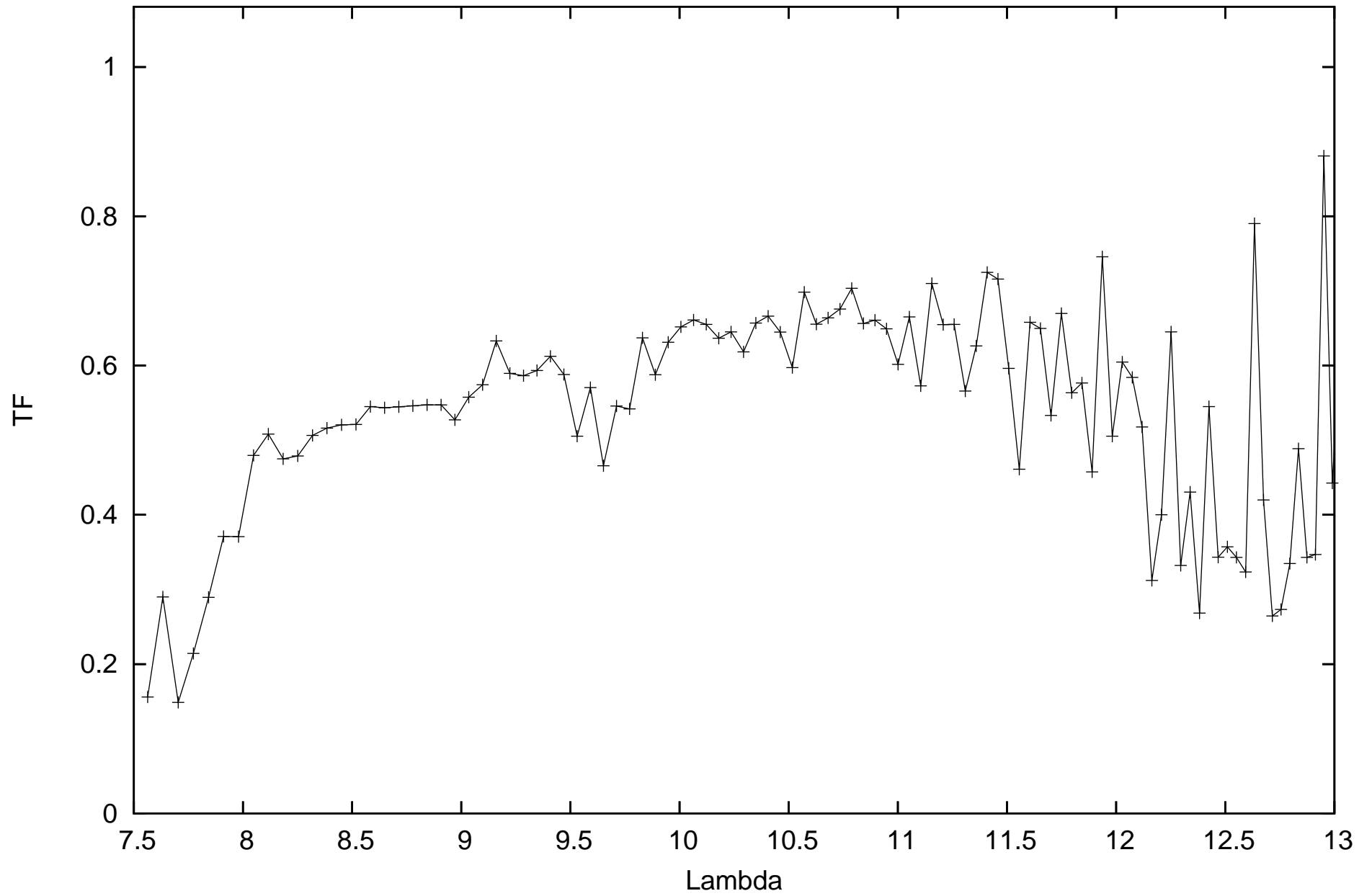
calHD206778_flux-1.04_diam7.59_r.MIDI.2011-05-09T09_50_58.945_C1B2
