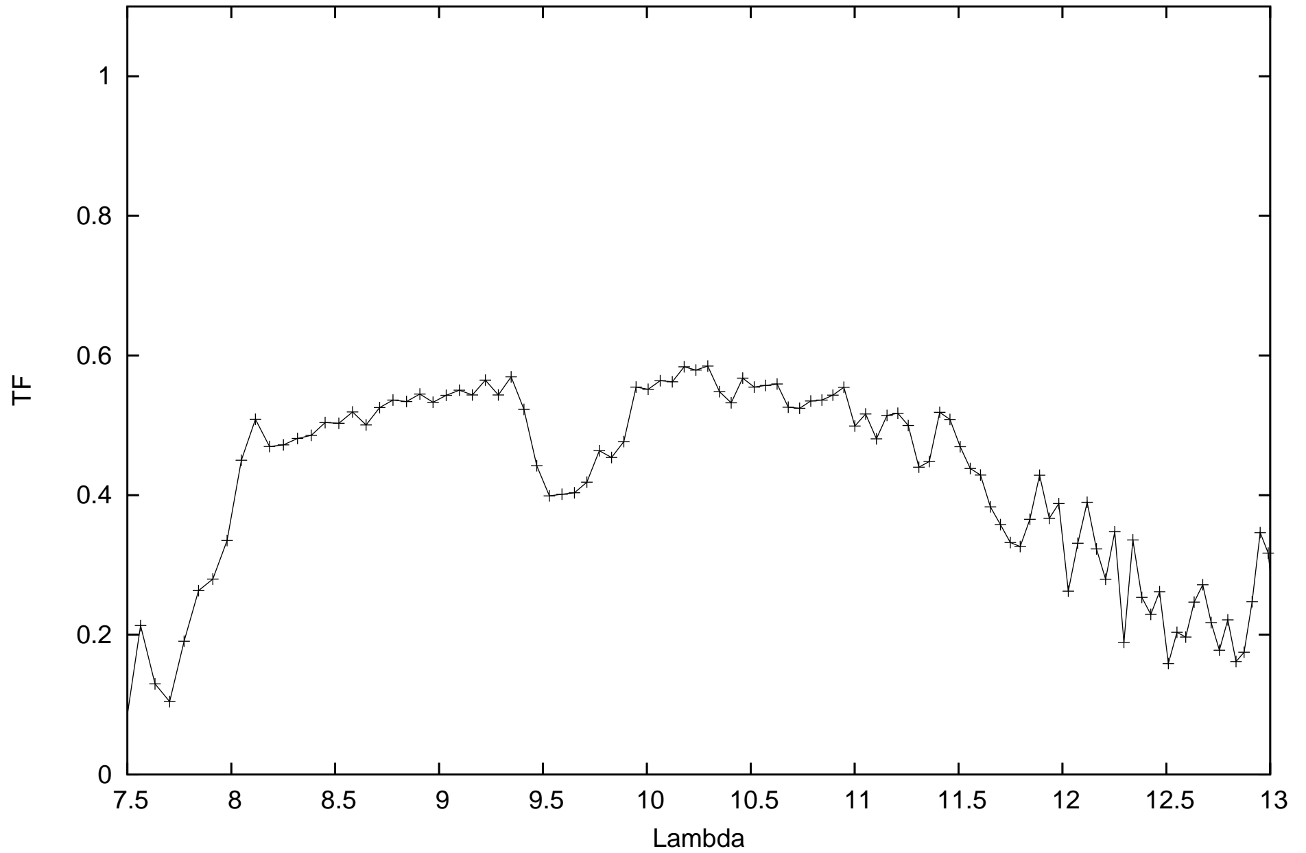
calHD206778_flux-1.04_diam7.59_r.MIDI.2011-05-09T09_19_12.946_C1B2
