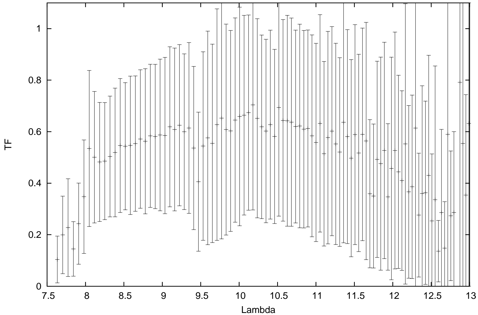
calHD206778_flux-1.04_diam7.59_r.MIDI.2011-05-09T08_45_29.180_C1B2
