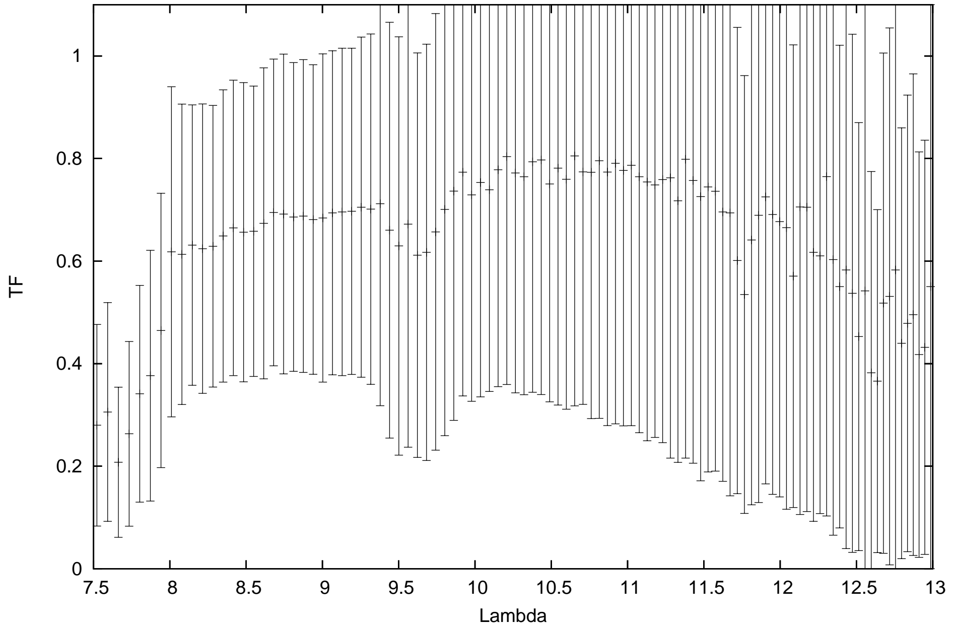
calHD107446_flux0.22_diam4.43_r.MIDI.2011-05-09T03_43_06.000_C1B2
