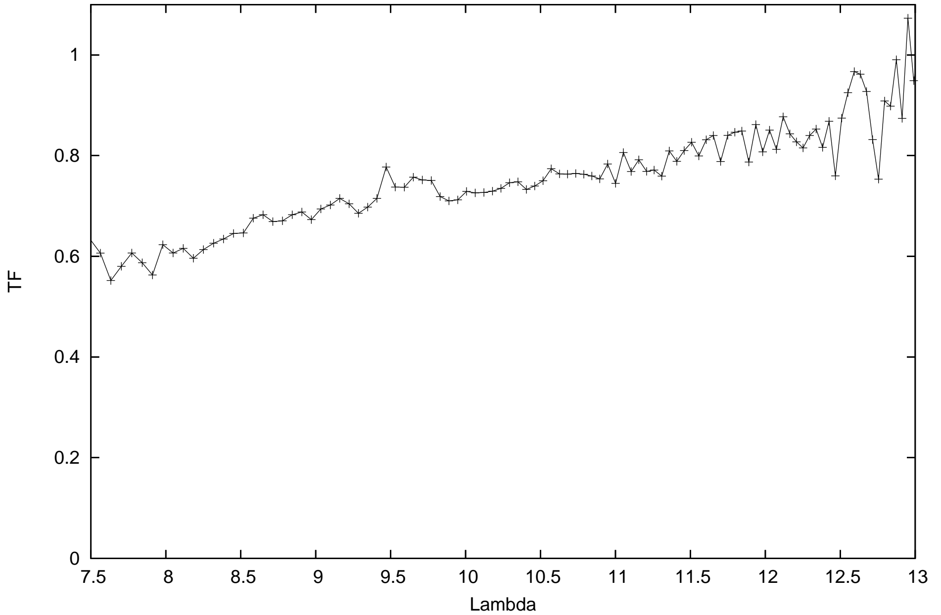
calHD120323_flux-2.02_diam13.25_r.MIDI.2011-05-07T01_34_08.945_C1A1
