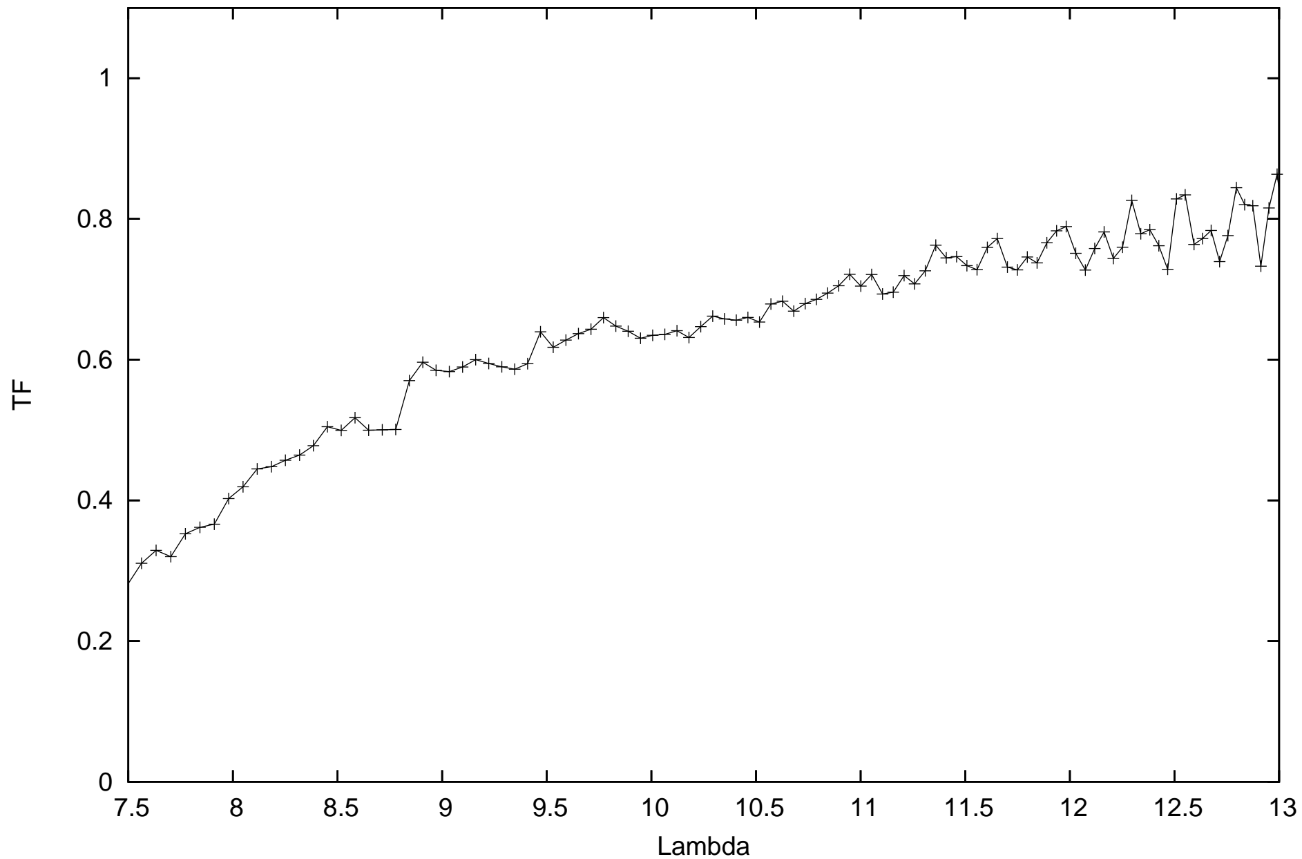
calHD120323_flux-2.02_diam13.25_r.MIDI.2011-03-08T04_17_51.015_H0G0
