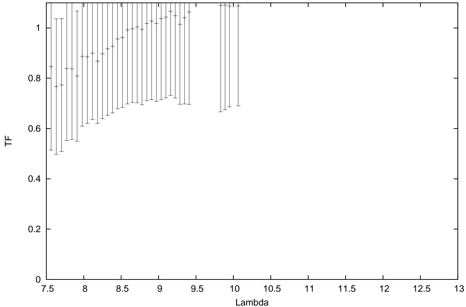
calHD167618_flux-1.82_diam11.66_r.MIDI.2011-03-06T09_25_09.138_H0G0
