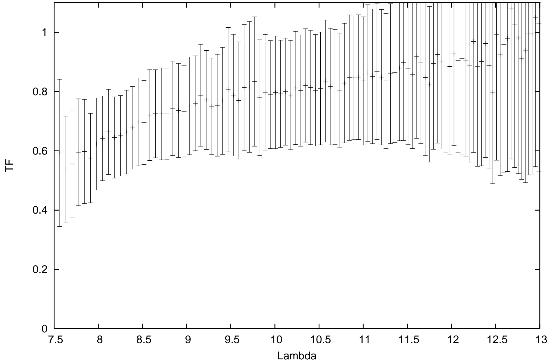
calHD167618_flux-1.82_diam11.66_r.MIDI.2011-03-05T09_13_47.137_G011
