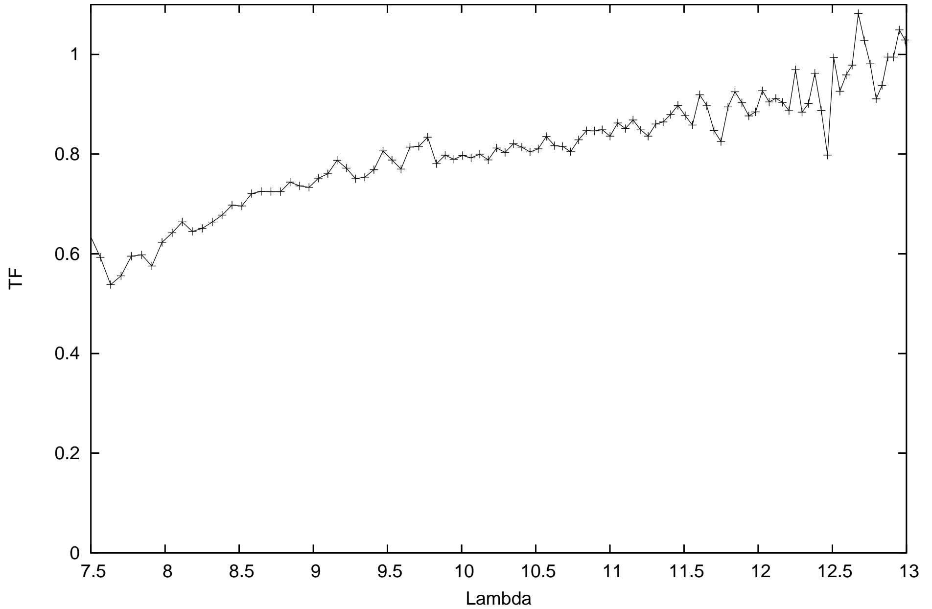
calHD167618_flux-1.82_diam11.66_r.MIDI.2011-03-05T09_13_47.137_G0I1
