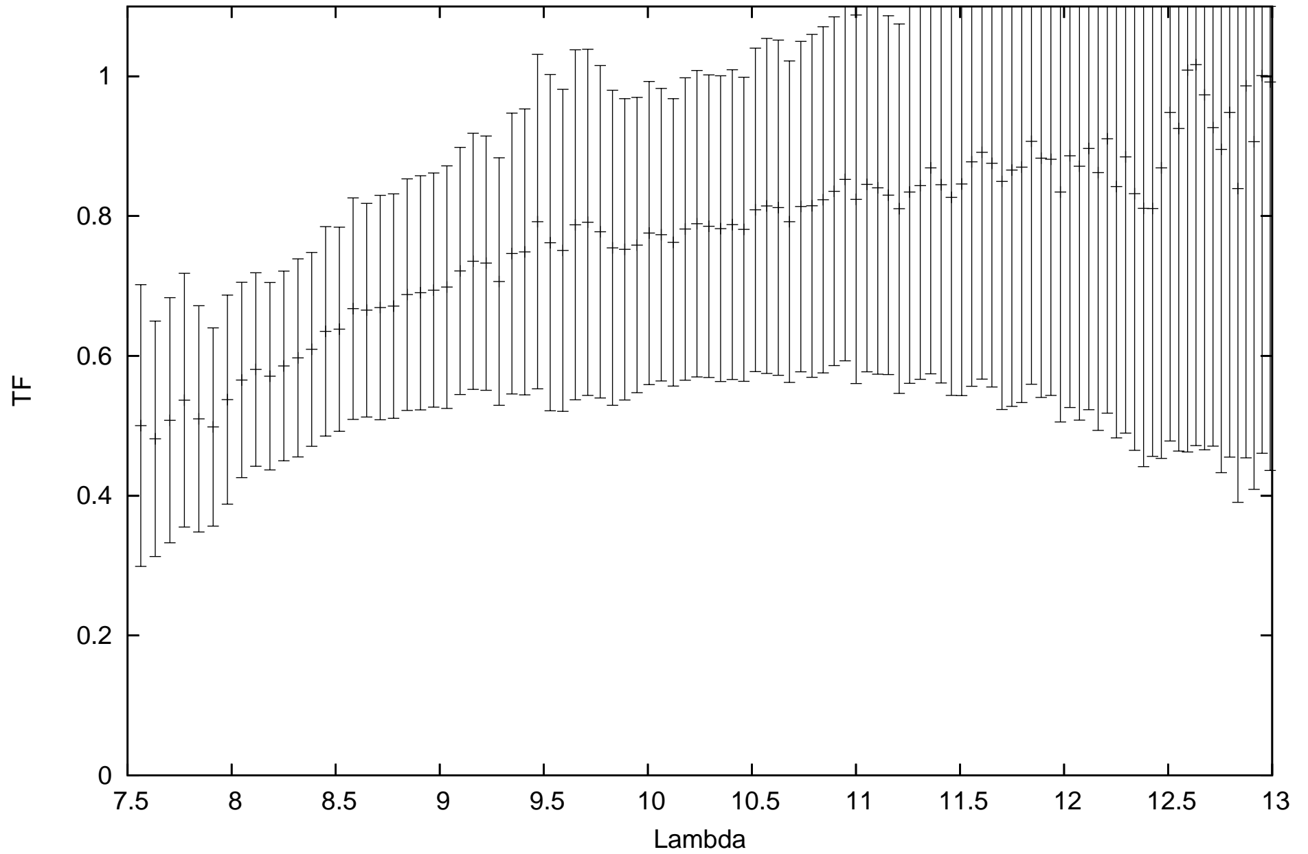
calHD133216_flux-1.76_diam11.15_r.MIDI.2011-03-05T08_31_07.137_I1E0
