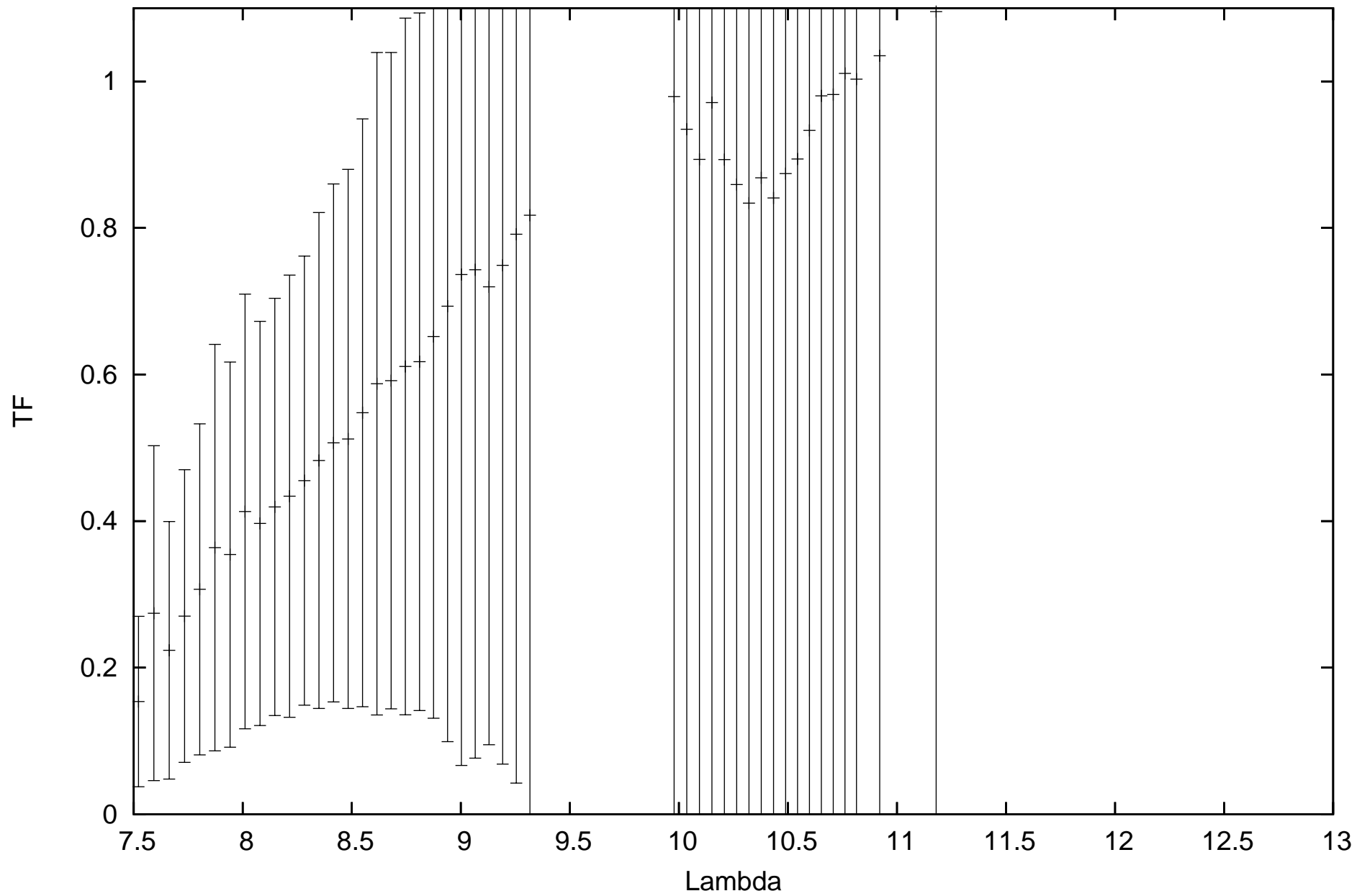
calHD133216_flux-1.76_diam11.15_r.MIDI.2011-02-27T06_57_59.000_D0B2
