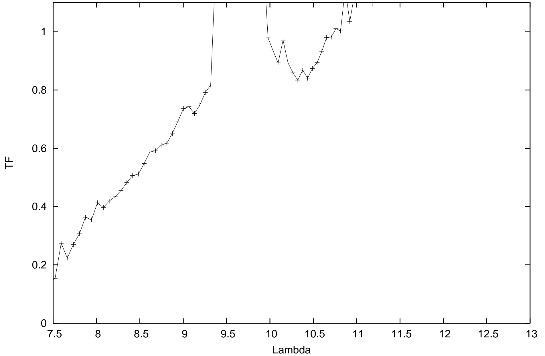
calHD133216_flux-1.76_diam11.15_r.MIDI.2011-02-27T06_57_59.000_D0B2
