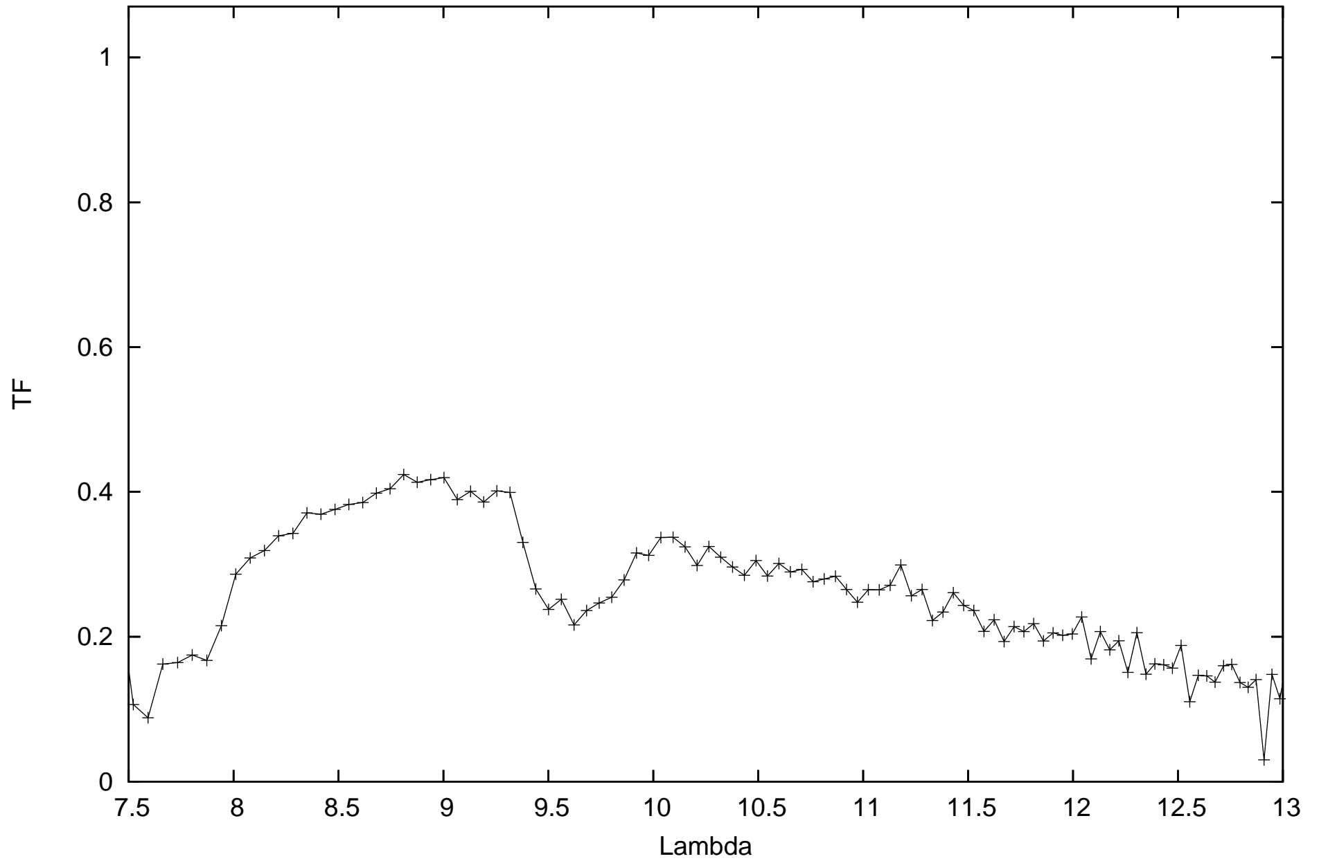
calHD123139_flux-0.39_diam5.34_r.MIDI.2011-02-27T06_43_36.000_D0B2
