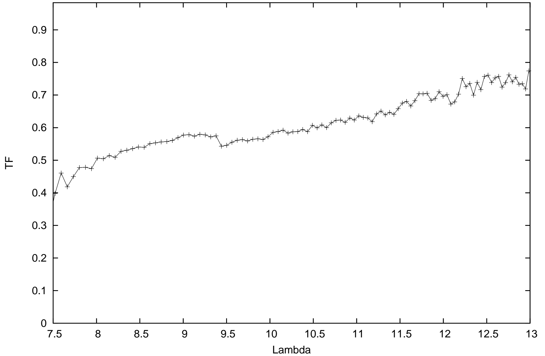
calHD120323_flux-2.02_diam13.25_r.MIDI.2011-02-27T07_17_57.000_D0B2
