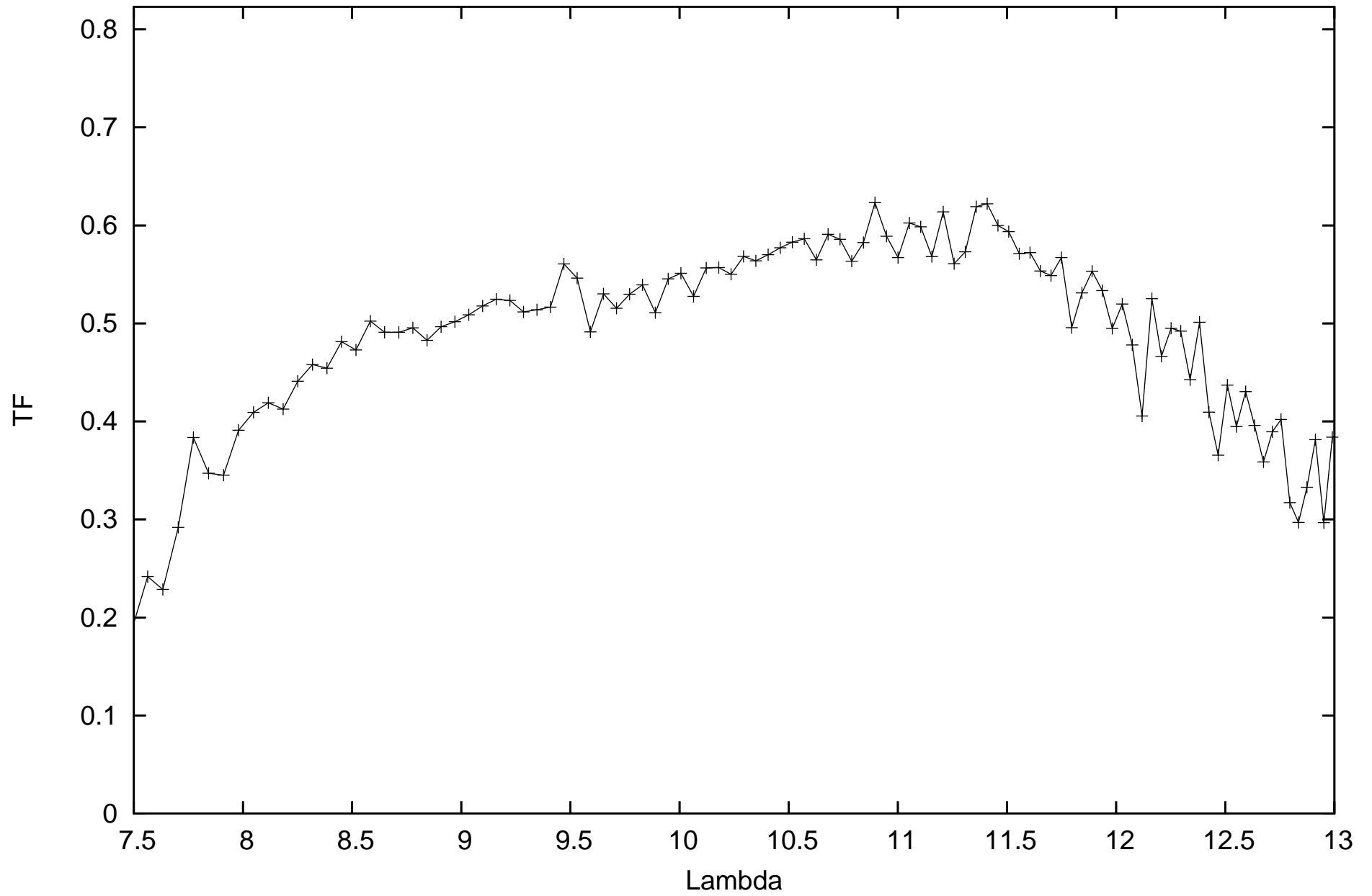
calHD081797_flux-1.49_diam9.14_r.MIDI.2011-02-27T05_06_52.138_B2A1
