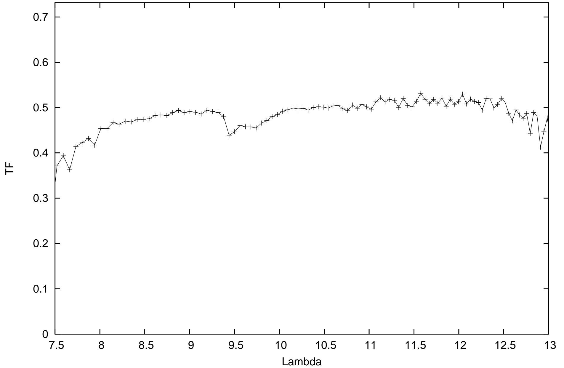
calHD081797_flux-1.49_diam9.14_r.MIDI.2011-02-27T04_58_13.000_B2A1
