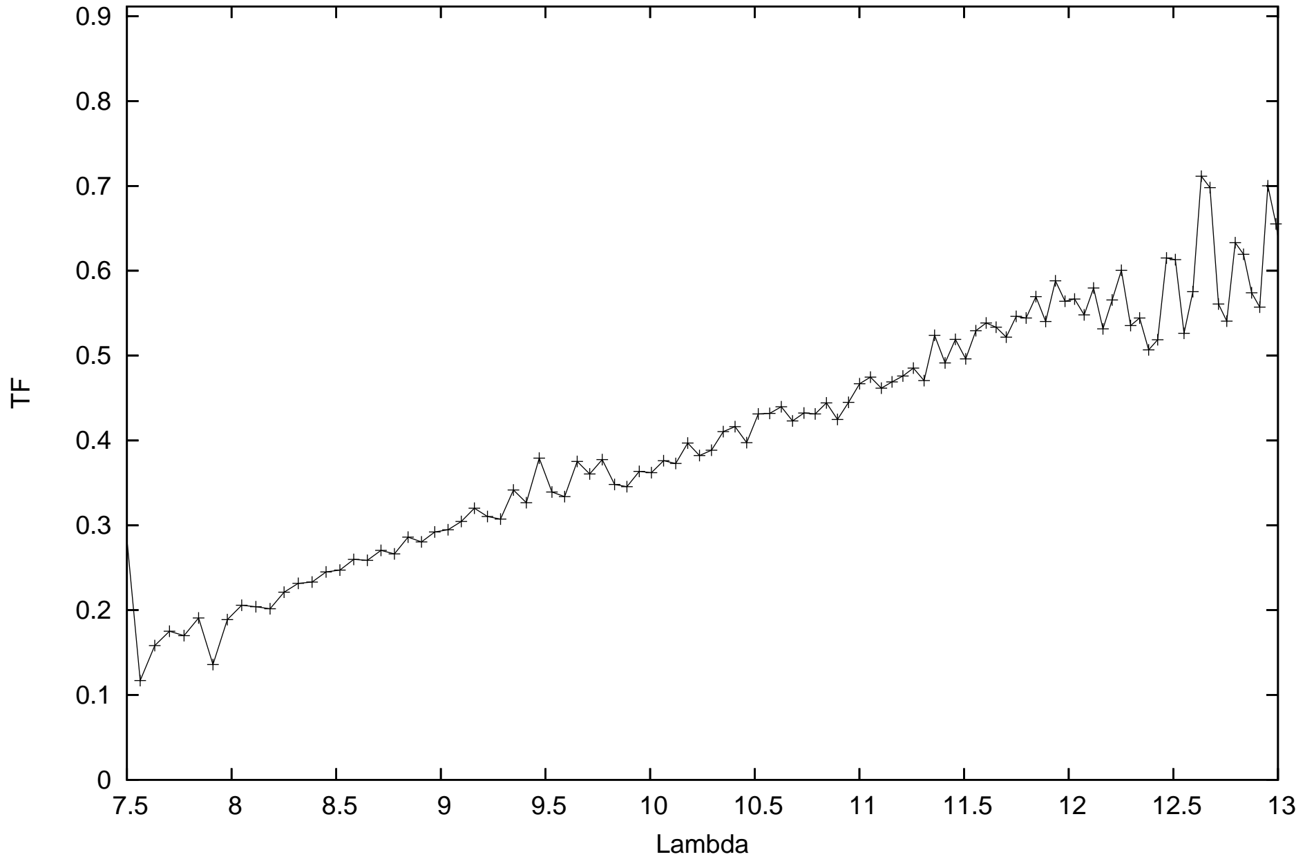
calHD133216_flux-1.76_diam11.15_r.MIDI.2011-02-11T08_40_13.138_H0G1
