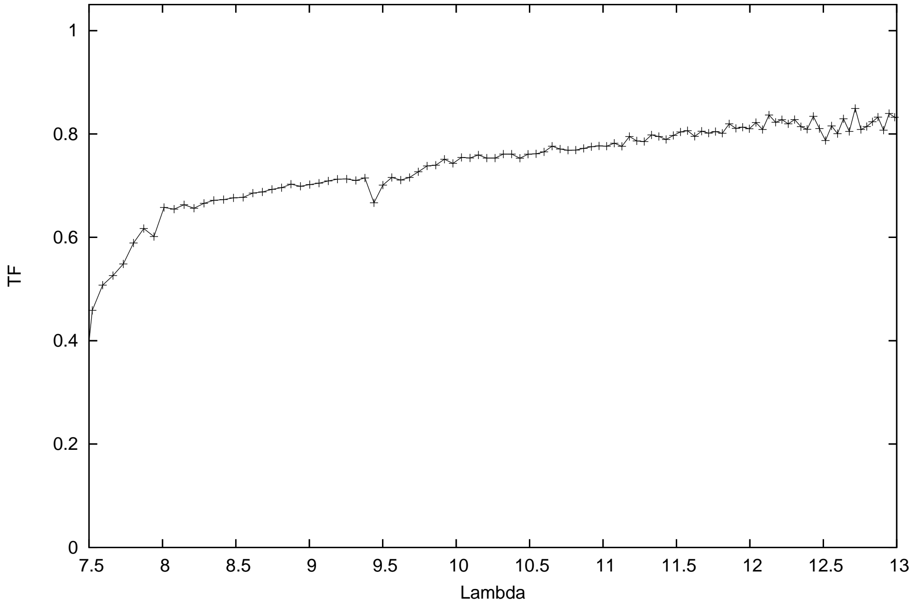
calHD120404_flux1.19_diam2.96_r.MIDI.2011-01-15T08_41_00.000_U3U4
