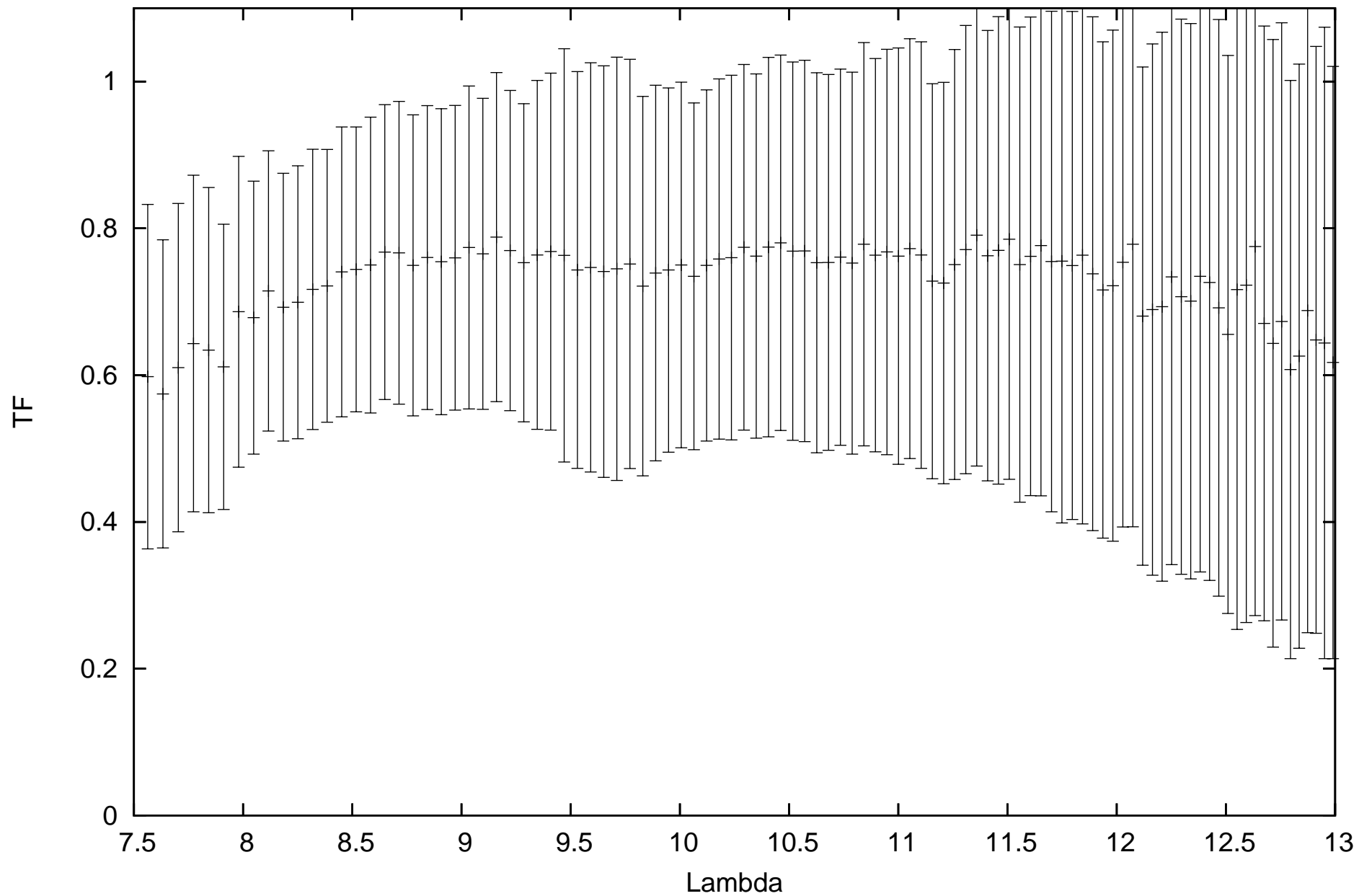
calHD081797_flux-1.49_diam9.14_r.MIDI.2011-01-10T08_10_59.138_DOC1
