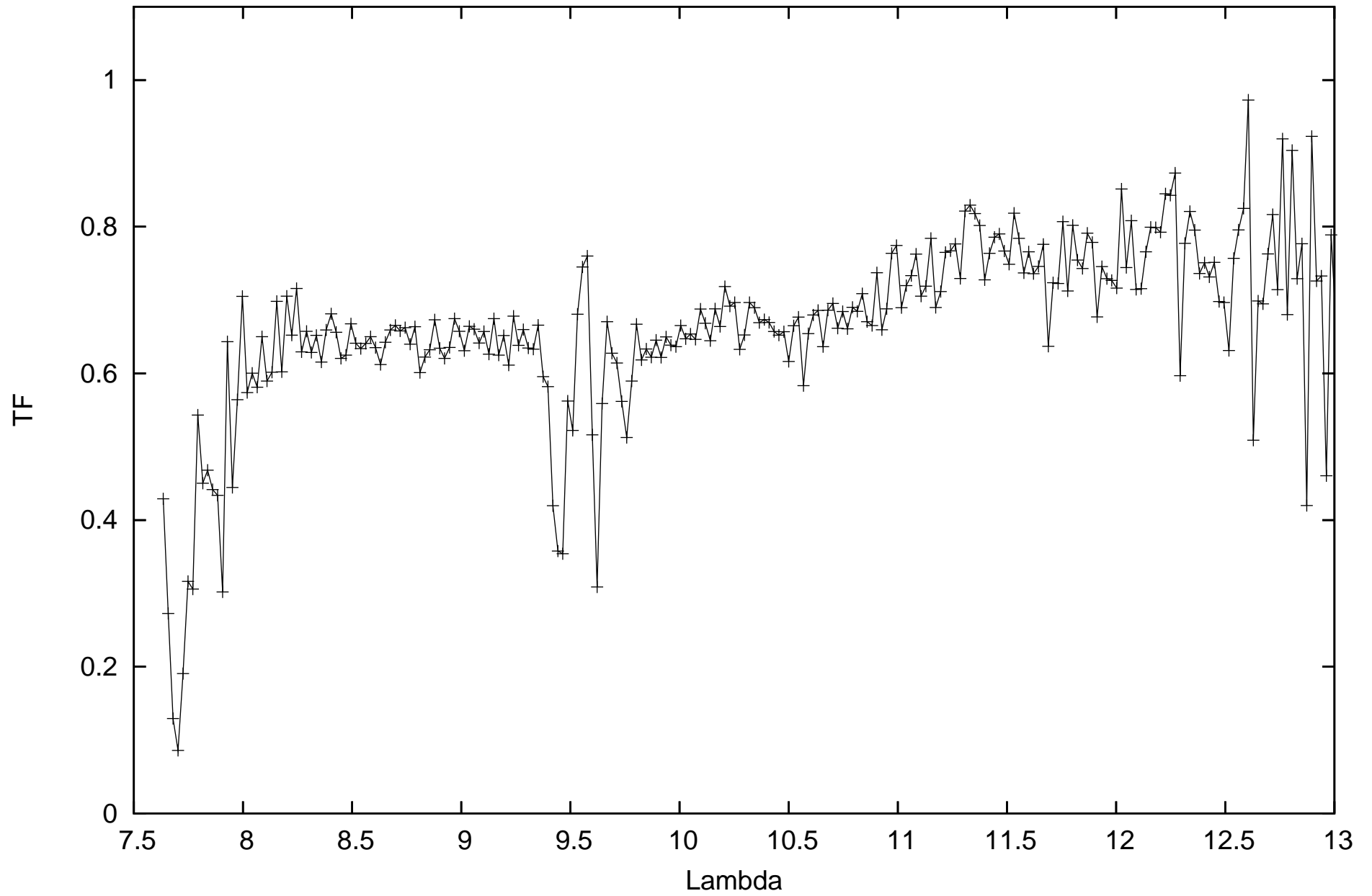
calHD206778_flux-1.04_diam7.59_r.MIDI.2010-10-09T01_08_10.389_D0H0
