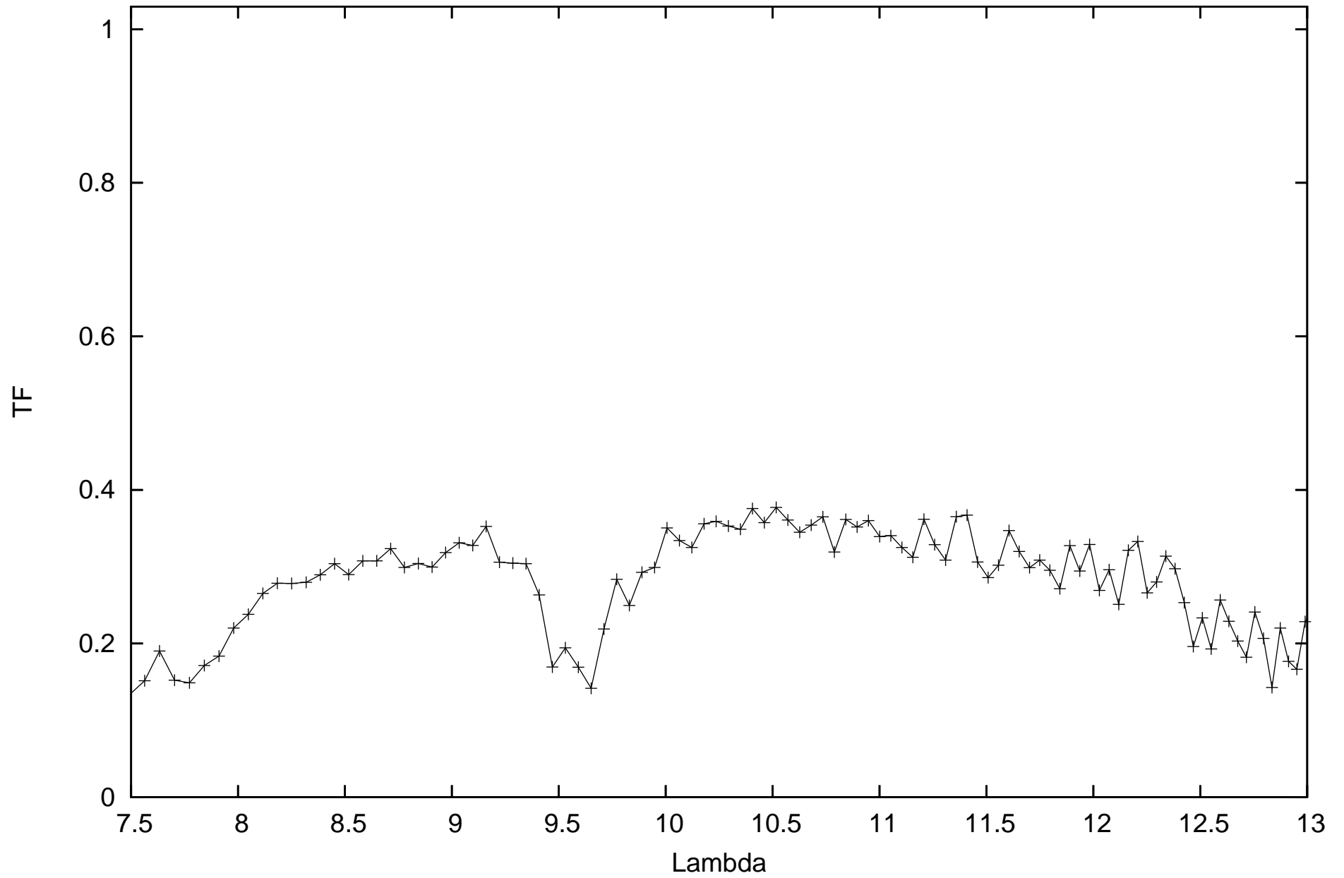
calHD206778_flux-1.04_diam7.59_r.MIDI.2010-10-07T03_39_48.179_G111
