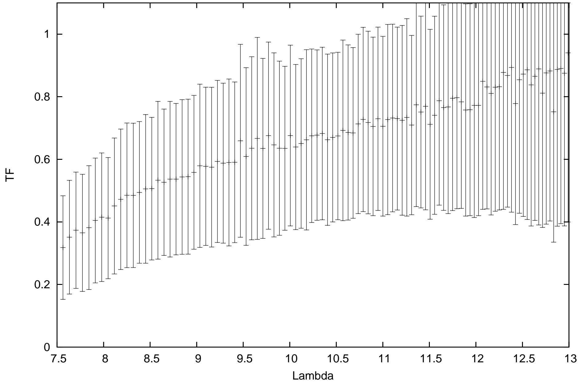
calHD167618_flux-1.82_diam11.66_r.MIDI.2010-10-01T00_44_30.138_K011
