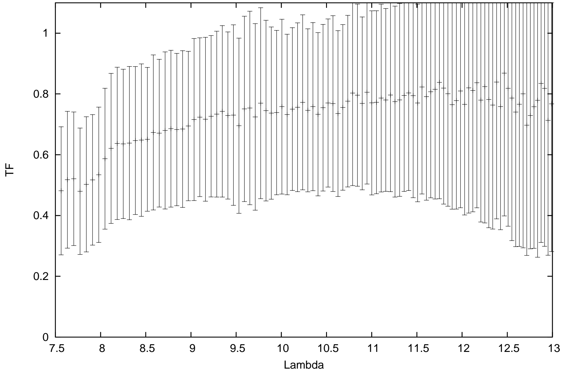
calHD167618_flux-1.82_diam11.66_r.MIDI.2010-09-24T00_13_51.138_C1A1
