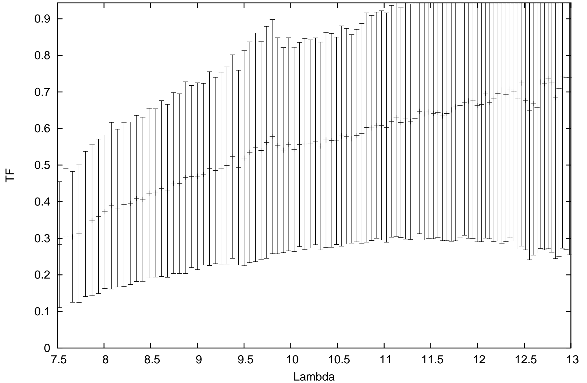
calHD206778_flux-1.04_diam7.59_r.MIDI.2010-08-22T04_00_19.000_H011
