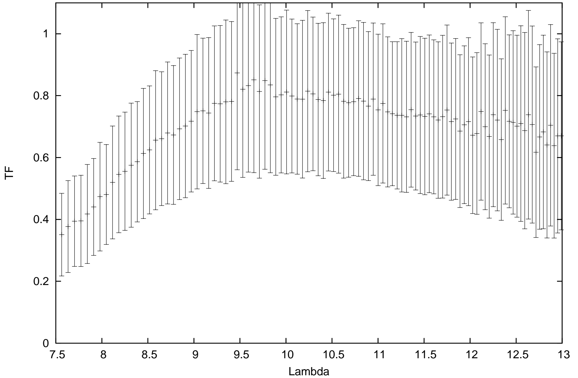
calHD167618_flux-1.82_diam11.66_r.MIDI.2010-08-22T02_19_16.138_H011
