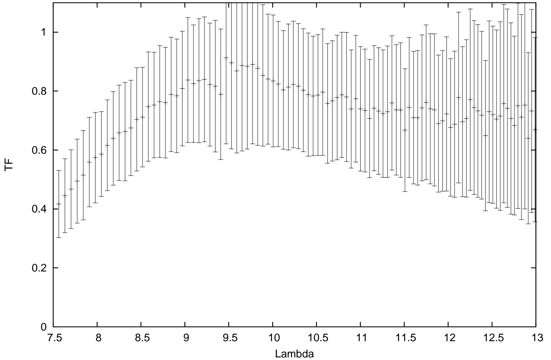
calHD167618_flux-1.82_diam11.66_r.MIDI.2010-08-21T04_18_12.138_H0I1
