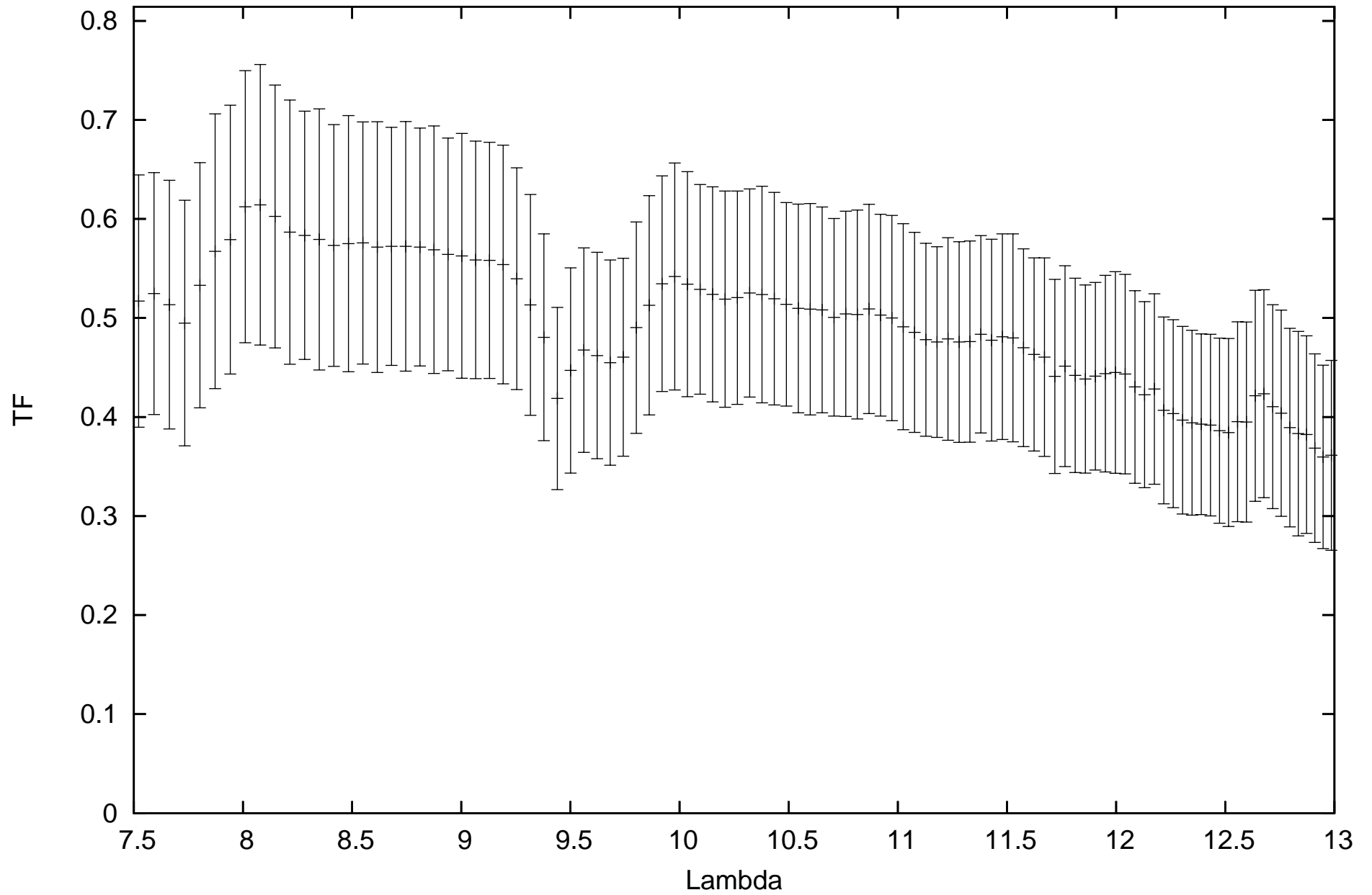
calHD167618_flux-1.82_diam11.66_r.MIDI.2010-08-21T04_09_36.000_H011
