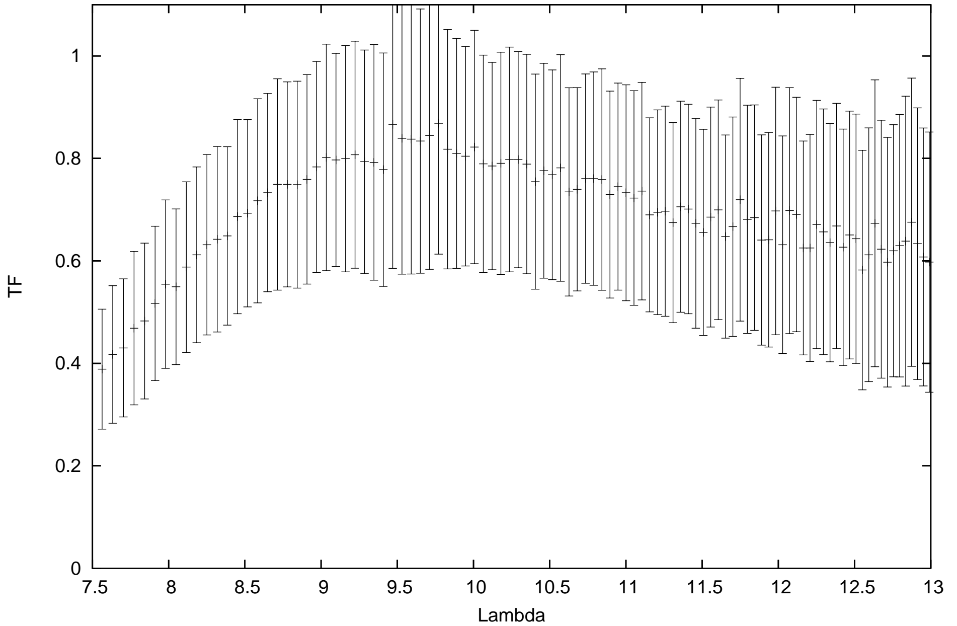
calHD167618_flux-1.82_diam11.66_r.MIDI.2010-08-21T03_52_01.138_H011
