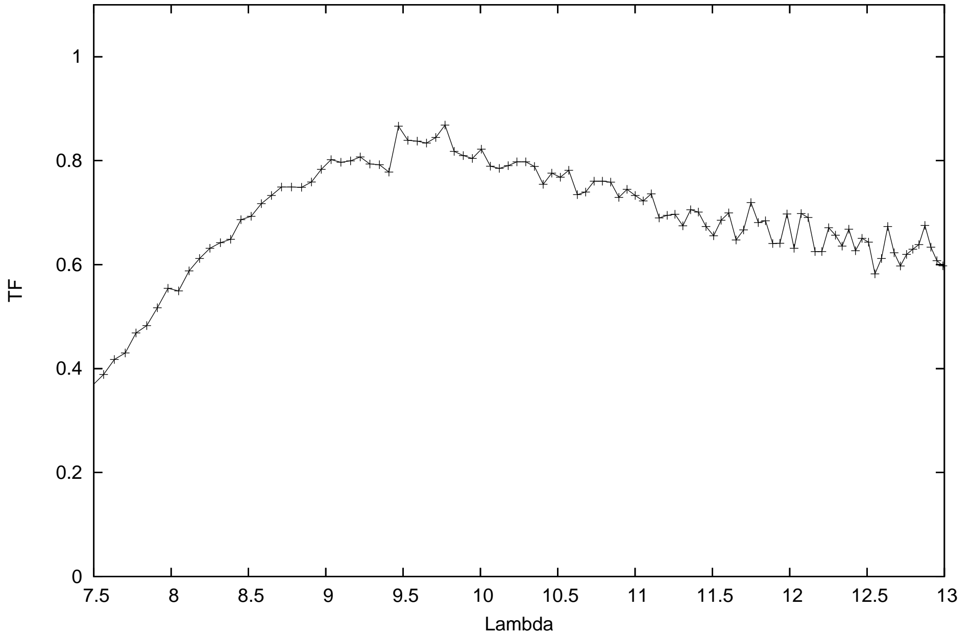
calHD167618_flux-1.82_diam11.66_r.MIDI.2010-08-21T03_52_01.138_H0I1
